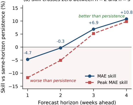
(a) Skill crosses zero between h = 2 and h = 3
