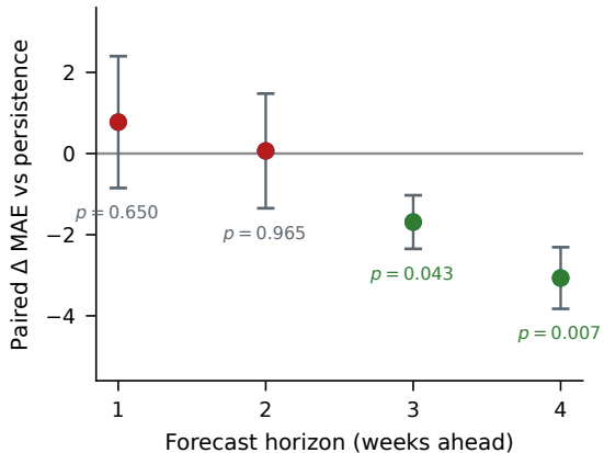
(b) Paired over 7 headline folds ( \pm s.e.)
