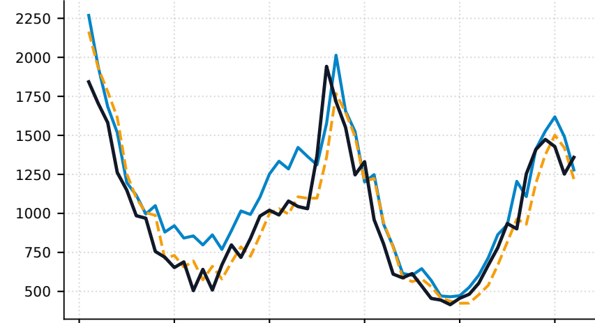
2021 (COVID) — NegBin: 94.5 | Quantile: 103.7 MAE
