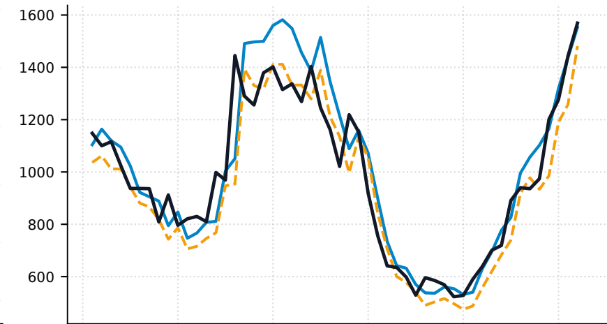
2025 — NegBin: 90.7 | Quantile: 86.7 MAE
