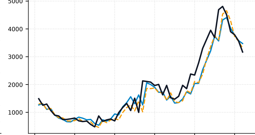
2022 — NegBin: 134.8 | Quantile: 129.6 MAE
