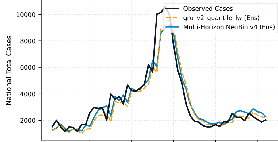
2020 (COVID) — NegBin: 124.3 | Quantile: 96.4 MAE
