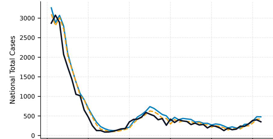
2023 — NegBin: 259.4 | Quantile: 253.8 MAE
