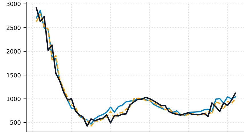
2024 — NegBin: 107.1 | Quantile: 92.0 MAE
