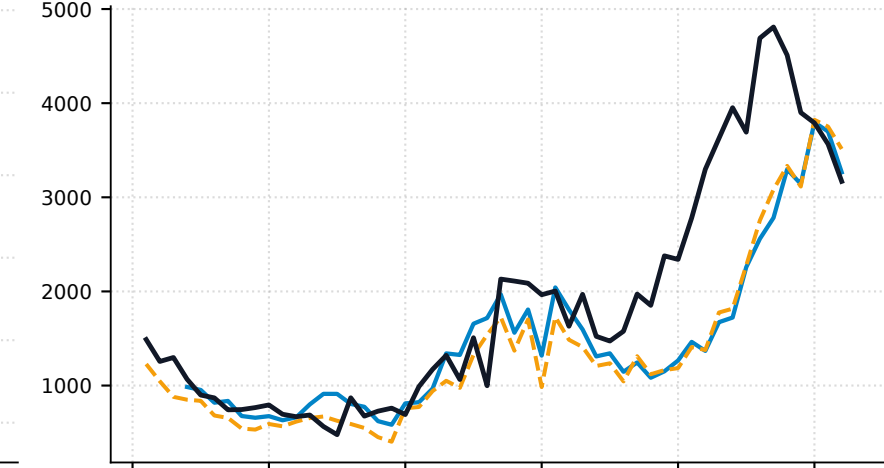
2022 — NegBin: 214.7 | Quantile: 192.6 MAE
