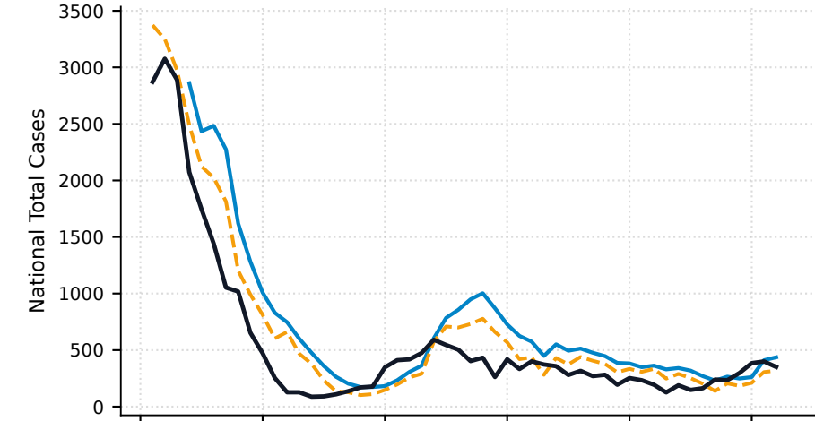
2023 — NegBin: 464.7 | Quantile: 448.4 MAE
