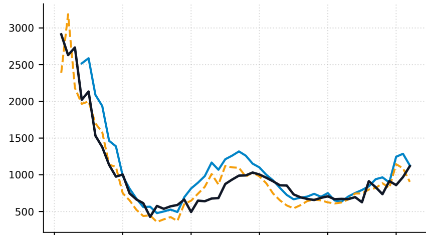
2024 — NegBin: 175.1 | Quantile: 125.0 MAE
