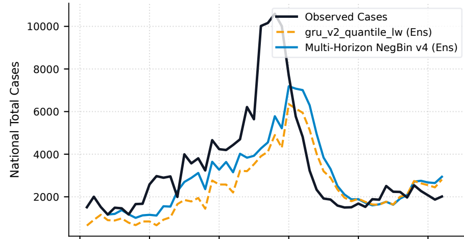
2020 (COVID) — NegBin: 292.5 | Quantile: 188.5 MAE
