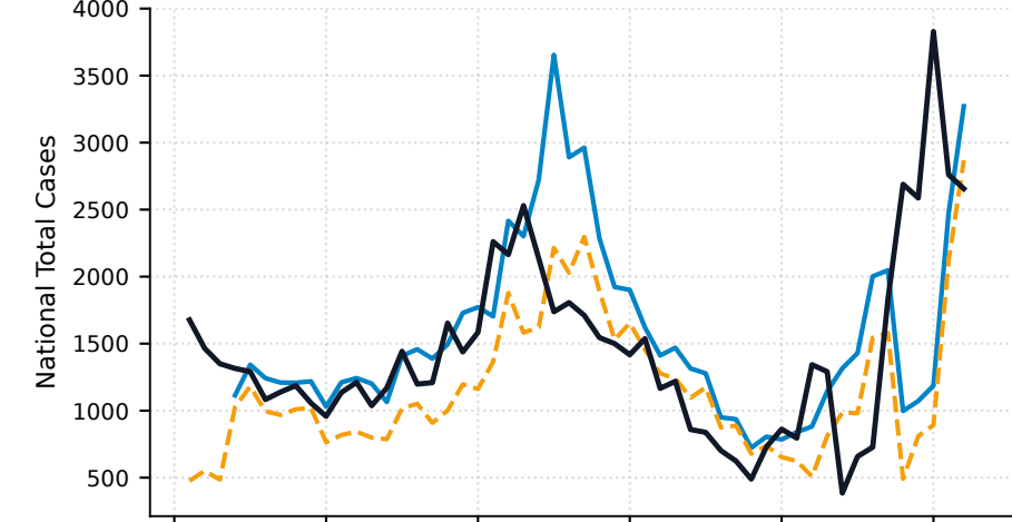
2023 — NegBin: 464.7 | Quantile: 448.4 MAE
