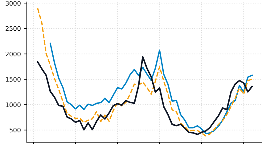
2021 (COVID) — NegBin: 165.2 | Quantile: 166.3 MAE
