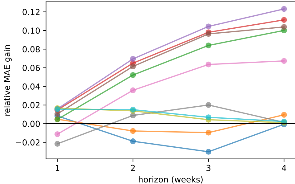
Case-only relative gain
