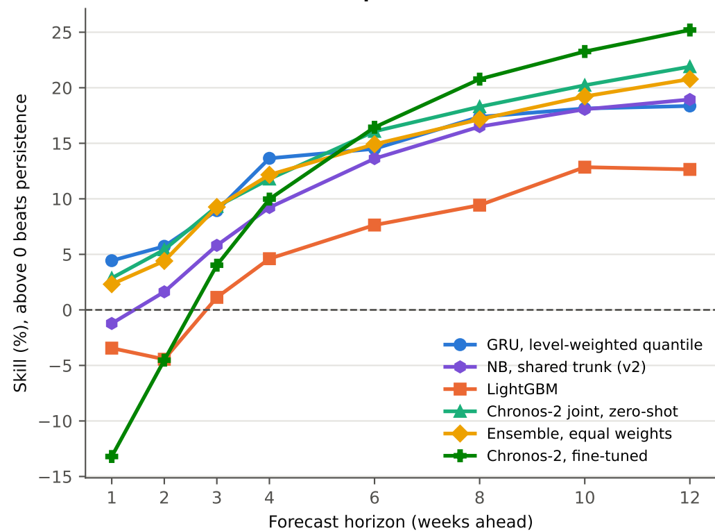
MAE skill vs same-horizon persistence (7 headline folds)
