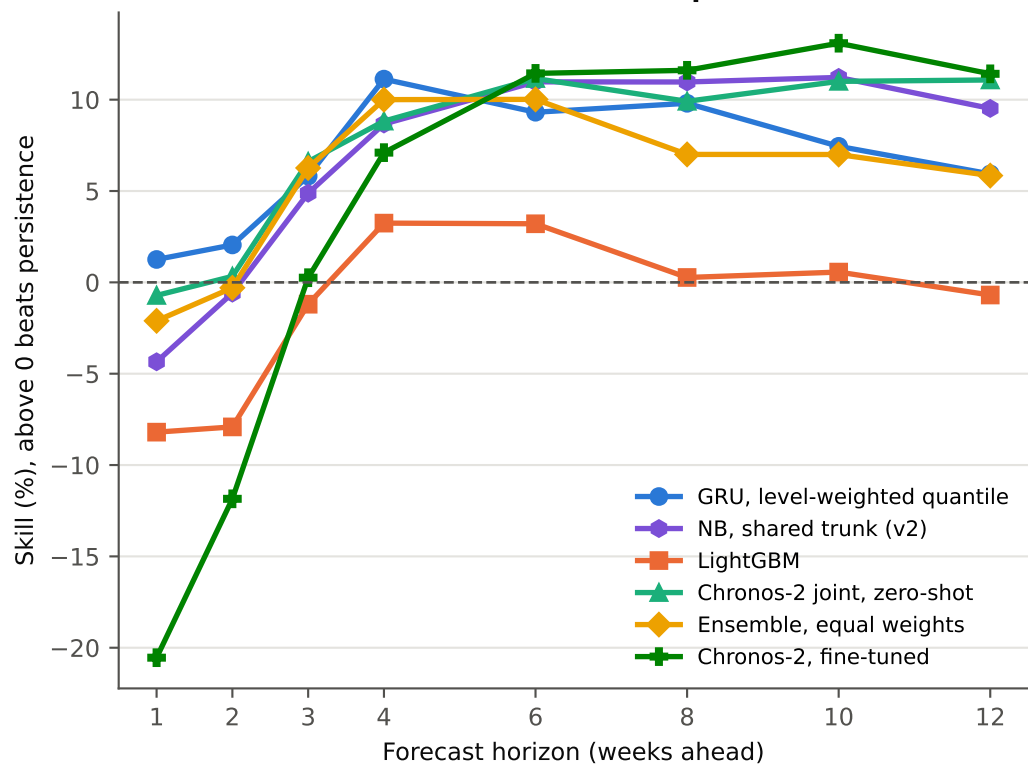
Peak-week MAE skill vs same-horizon persistence (7 headline folds)
