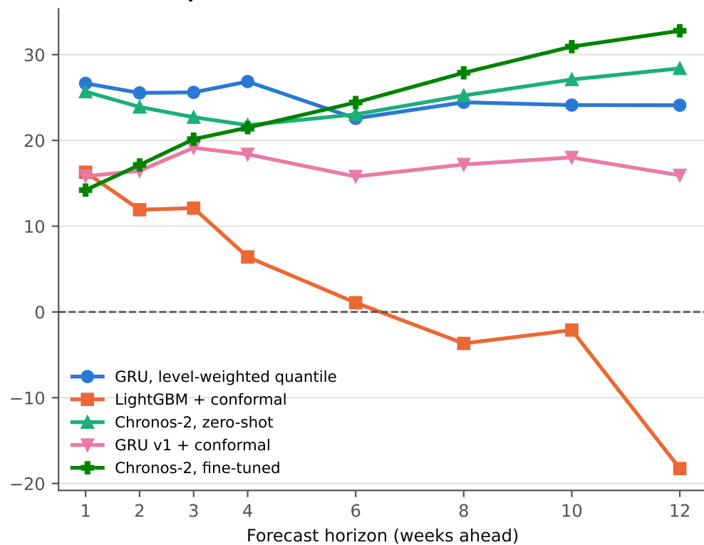
WIS skill vs persistence with conformal intervals
