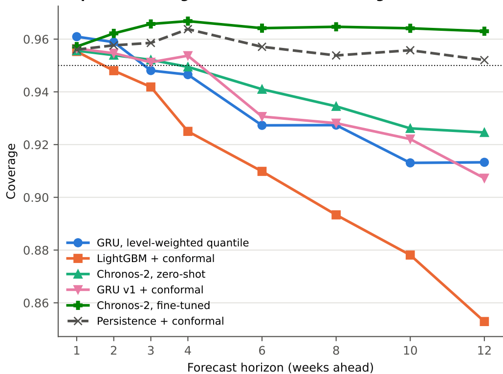
Empirical coverage of the 95% interval (target 0.95)
