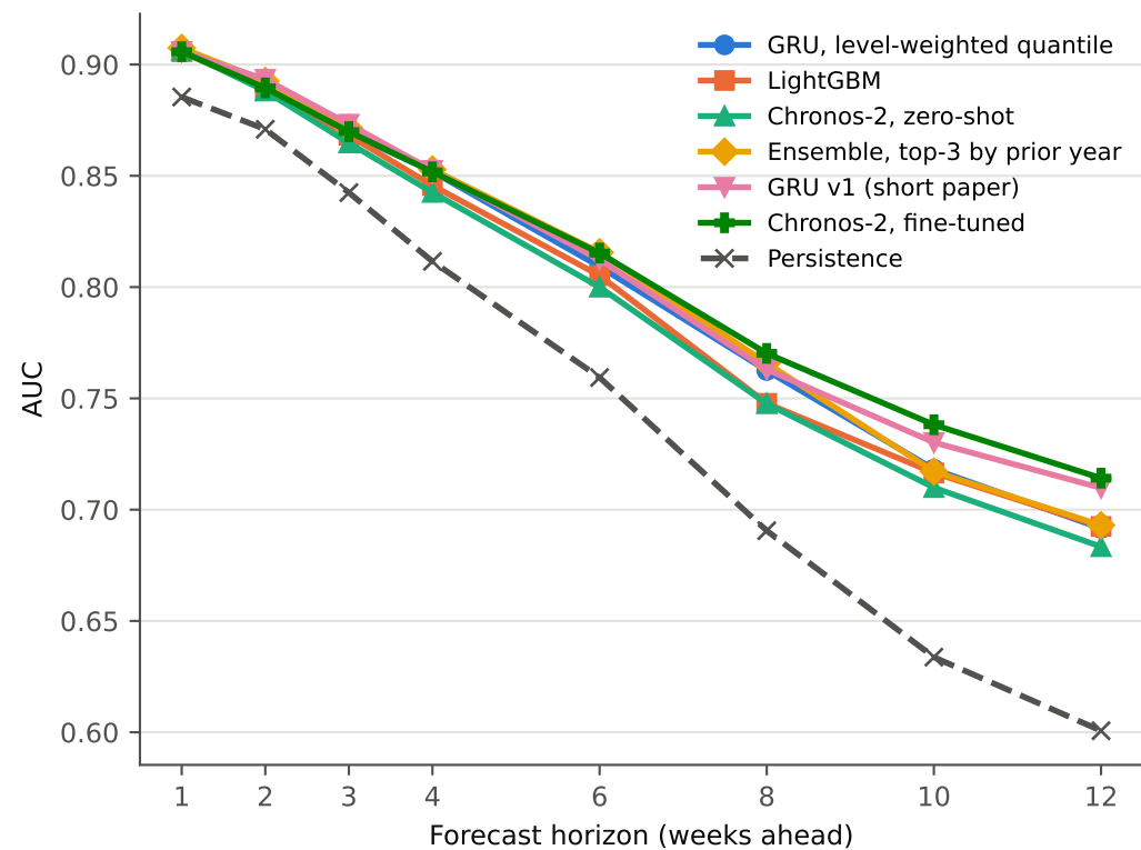
Outbreak weeks vs all other weeks (ROC-AUC)
