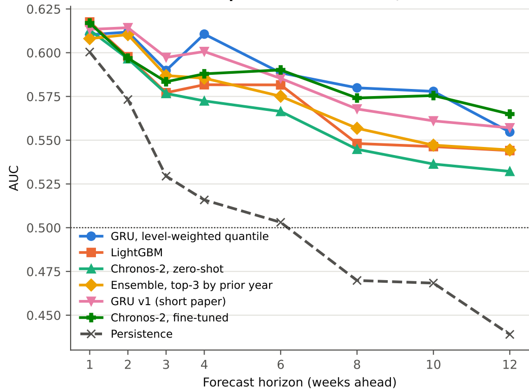
Outbreak onsets vs quiet weeks (ROC-AUC; 0.5 = chance)
