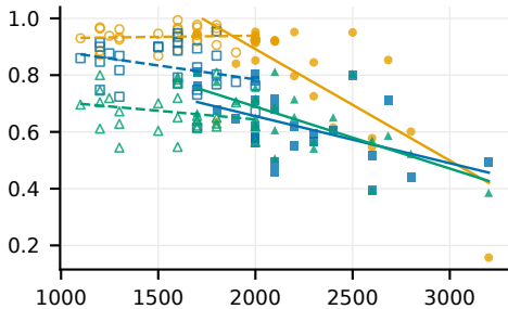
Task B: repair success
