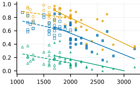
Task C: behavior preserved
