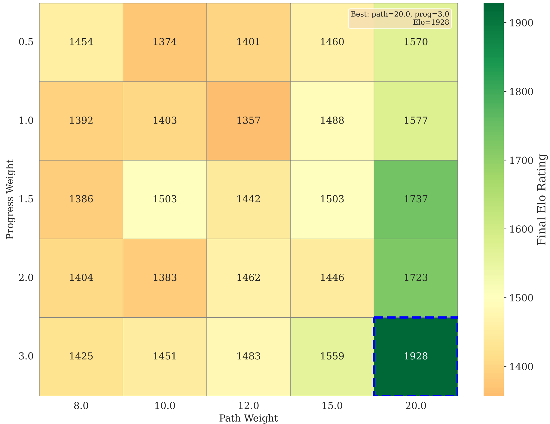
Hyperparameter Performance (Wall Weight = 1.0)
