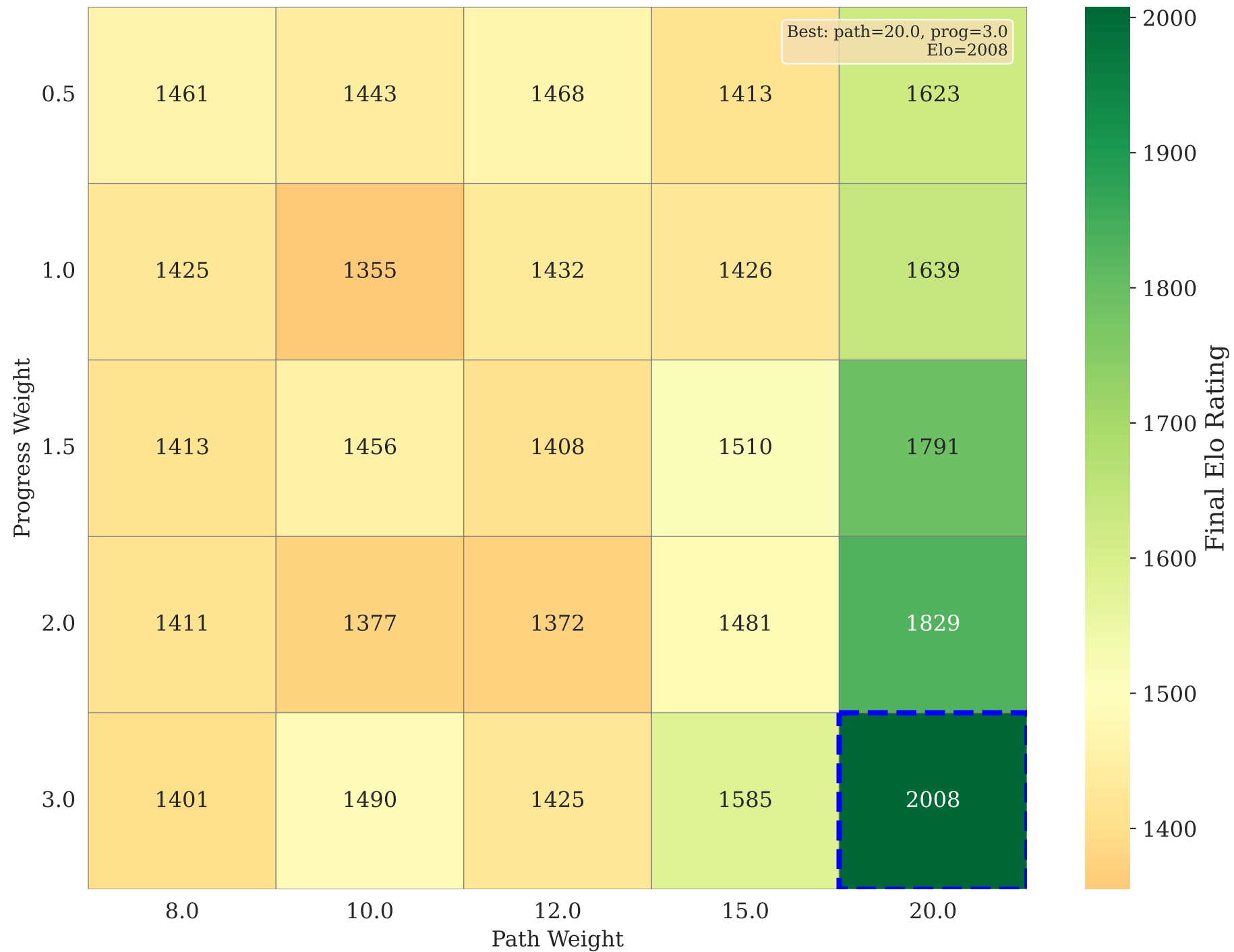
Hyperparameter Performance (Wall Weight = 3.0)
