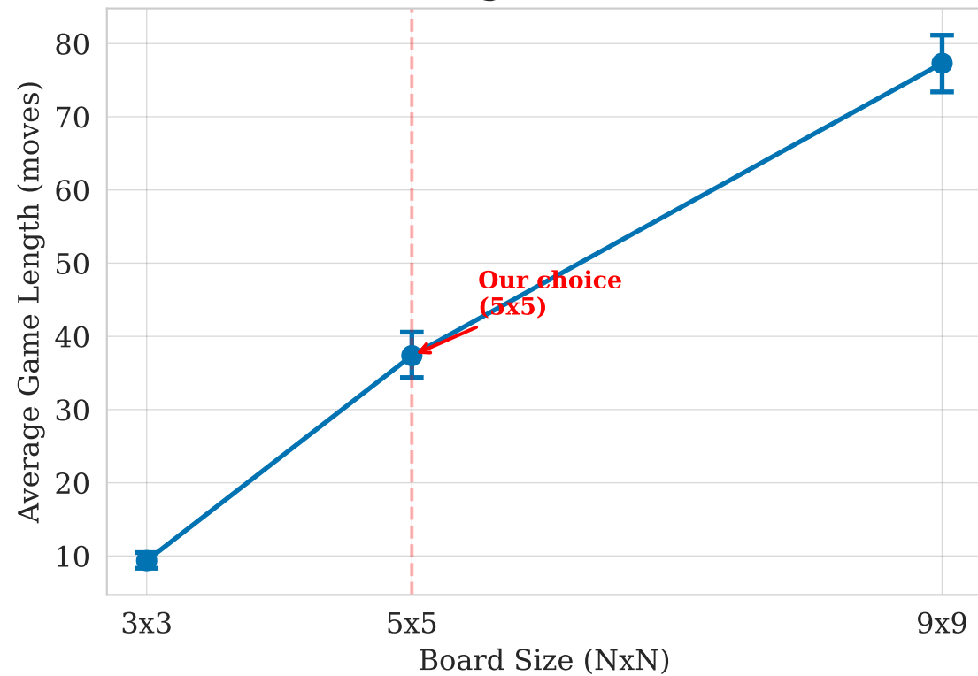
Game Length vs Board Size
