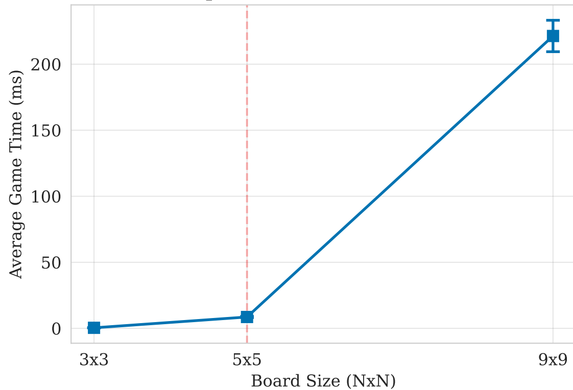
Computation Time vs Board Size
