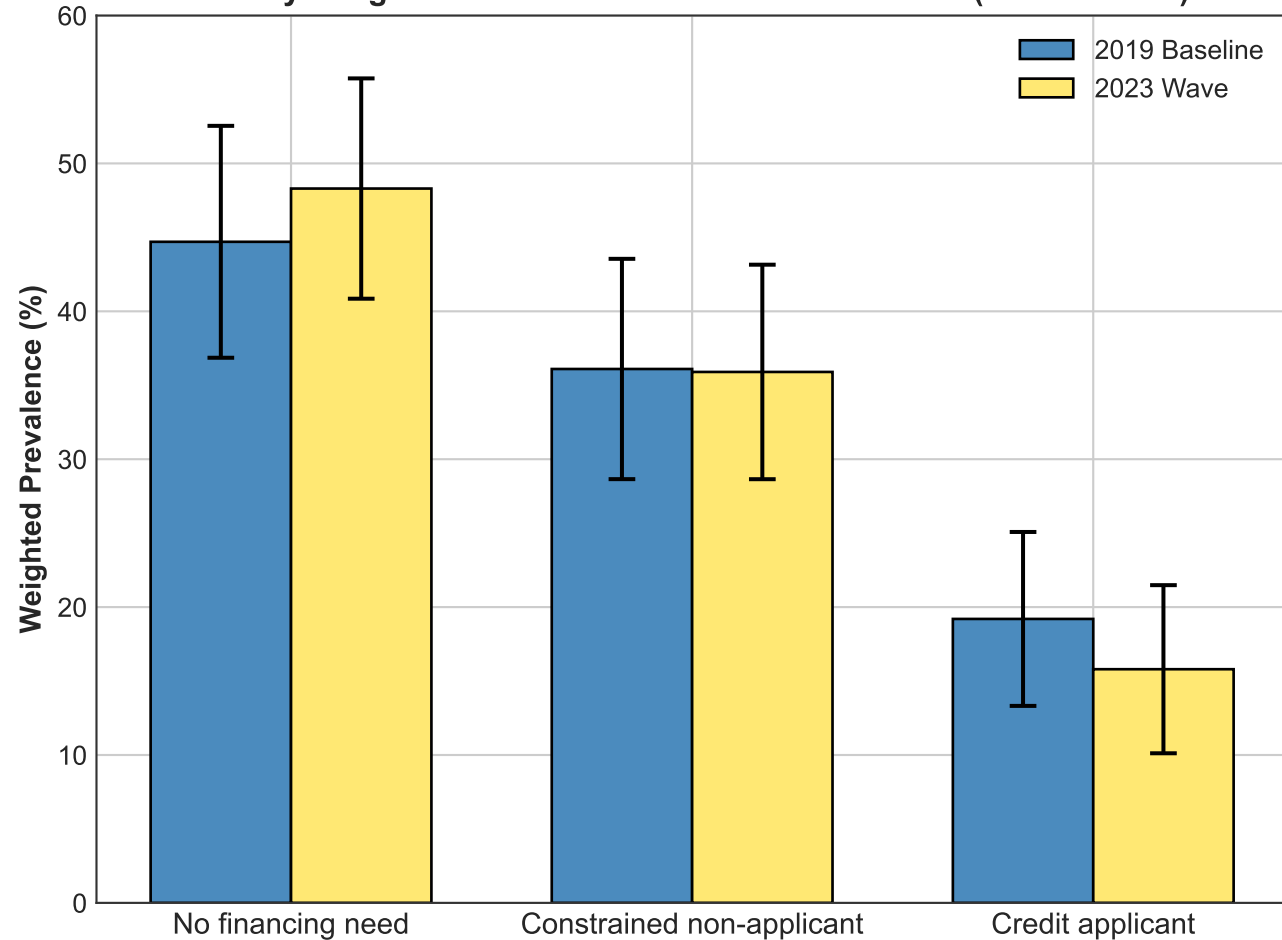
Survey-Weighted Credit-Market State Distributions (2019 vs 2023)
