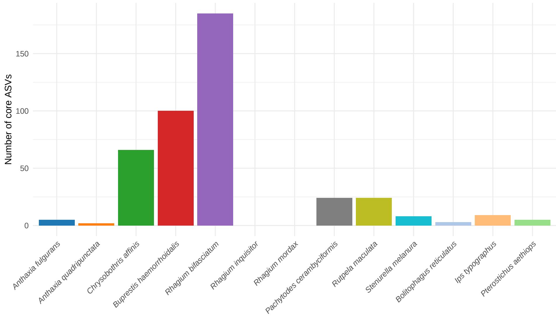
Core mycobiome size per beetle species (prevalence = 70%)
