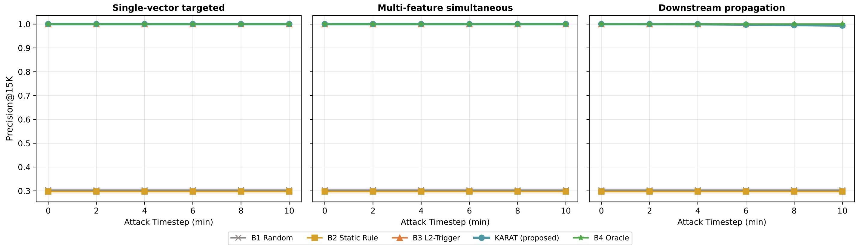
Figure 2: KARAT vs Baselines — Precision@15K Under Attack (5-seed mean \pm std)
