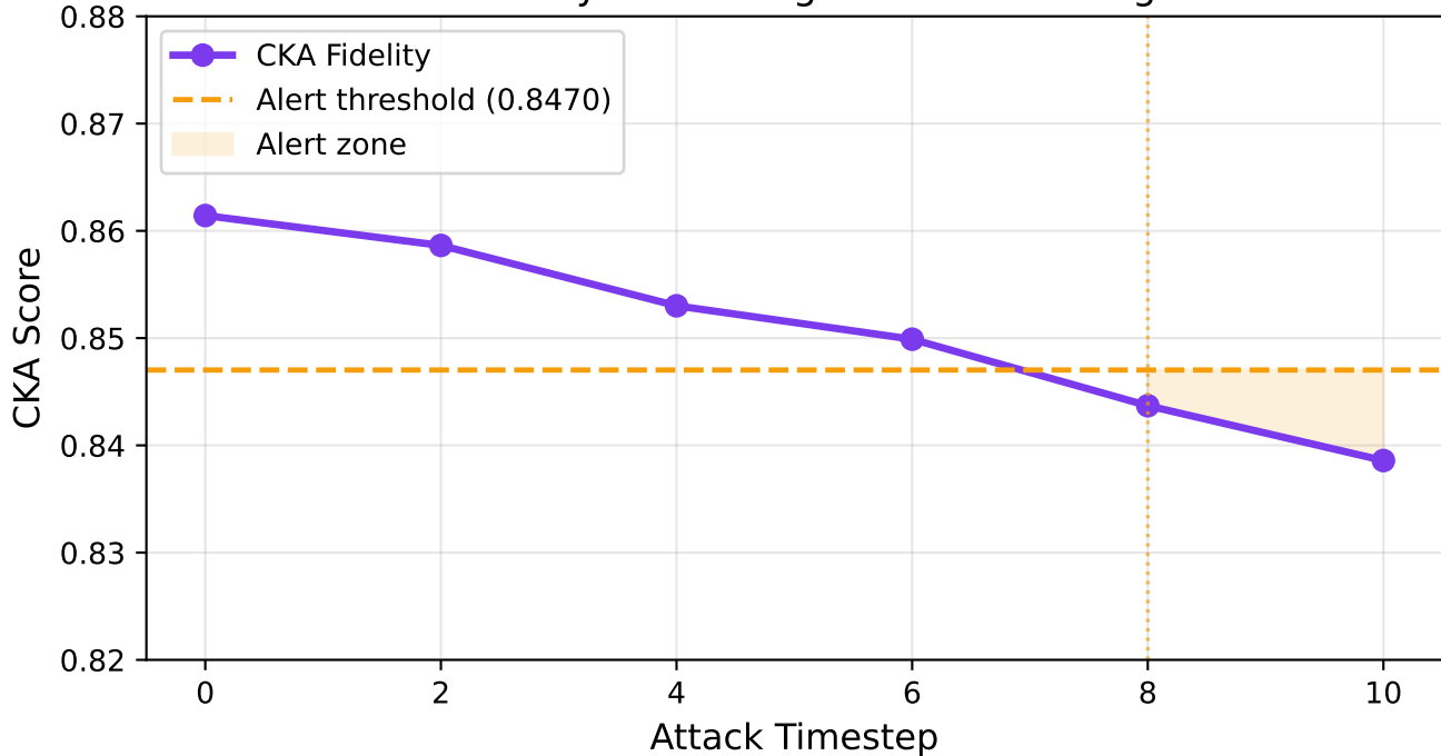
E1: CKA Fidelity Monitoring Under Escalating Attack
