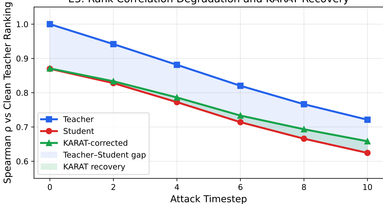
E3: Rank Correlation Degradation and KARAT Recovery
