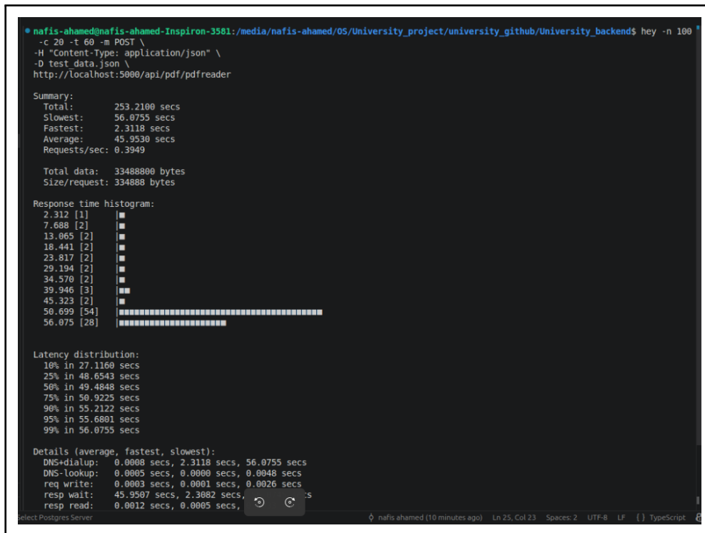
Figure 4.1: Load Testing Result Overview
