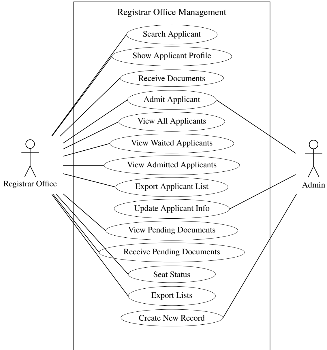
Figure 2.5: Use Case Diagram of Registrar Office Management
