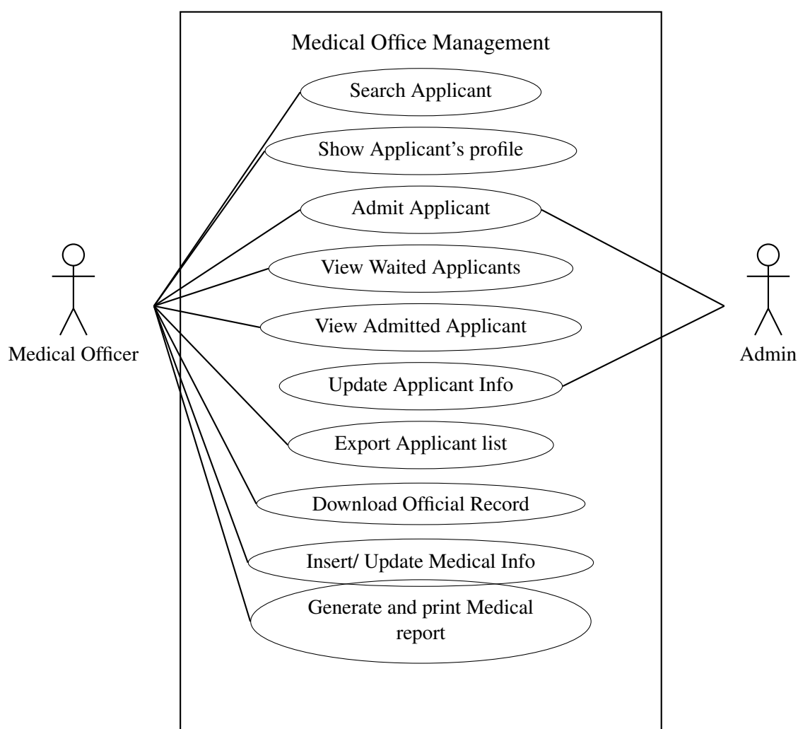
Figure 2.4: Use Case Diagram of Medical Office Management
