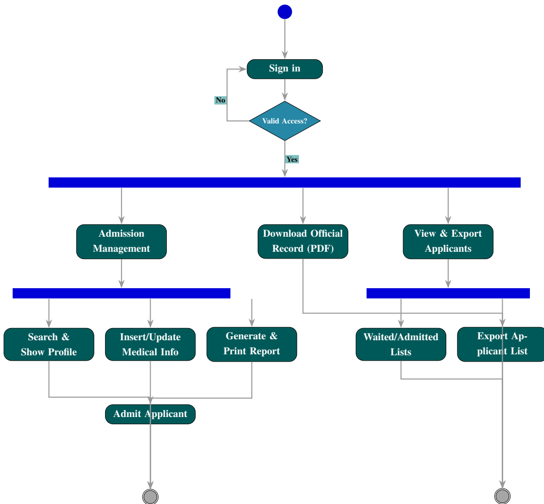
Figure 2.10: Activity Diagram of Medical Office Management (UC-4.0)
