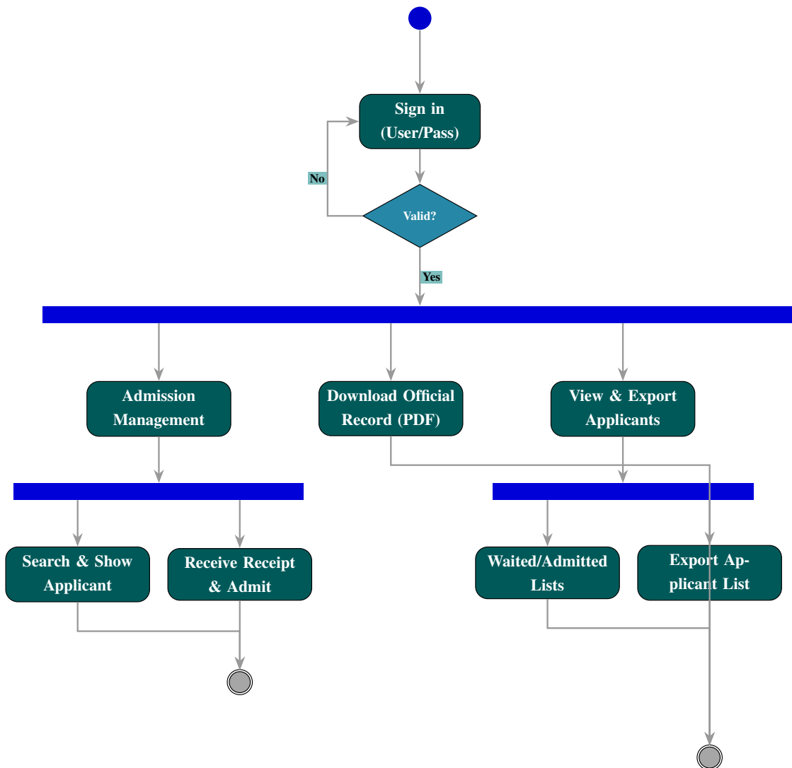
Figure 2.9: Activity Diagram of Hall Office Management (UC-6.0)
