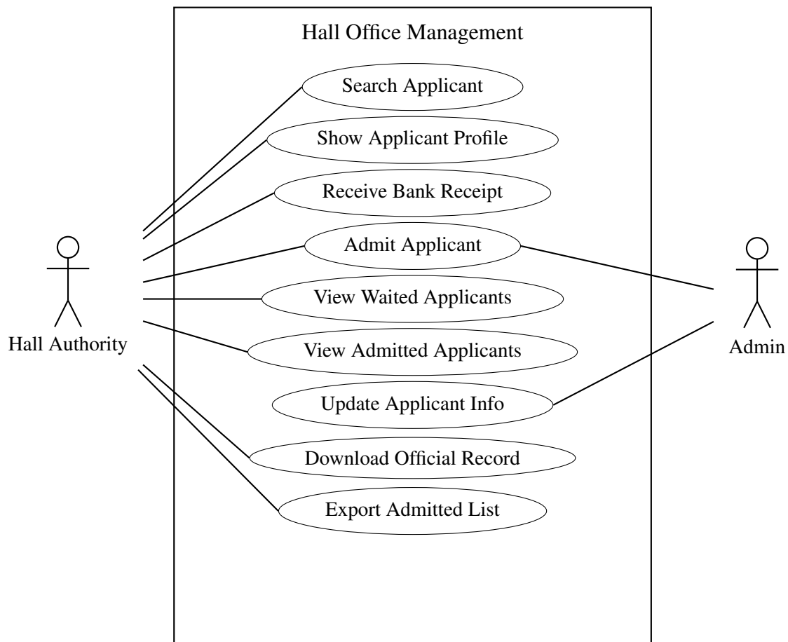
Figure 2.3: Use Case Diagram of Hall Office Management
