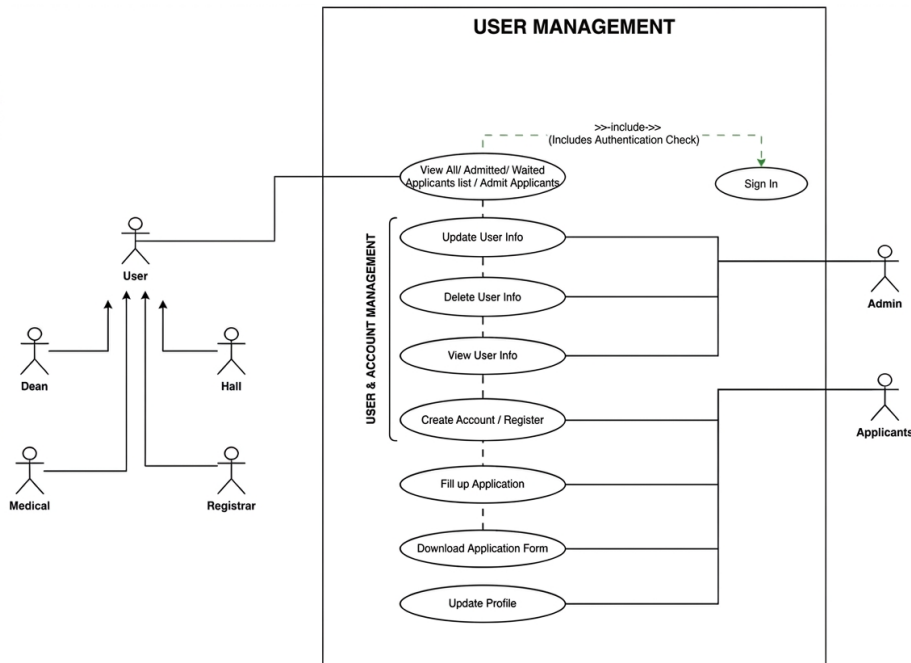
Figure 2.1: Use Case Diagram of User Management
