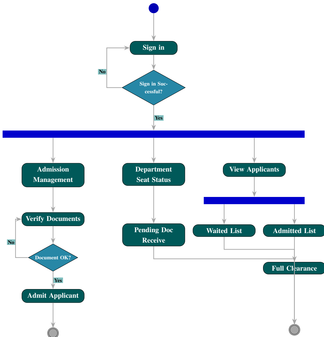
Figure 2.8: Activity Diagram of Dean Office Management (UC-5.0)
