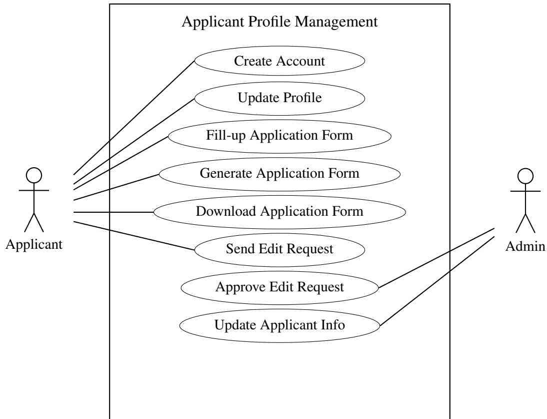
Figure 2.6: Use Case Diagram of Applicant Profile Management
