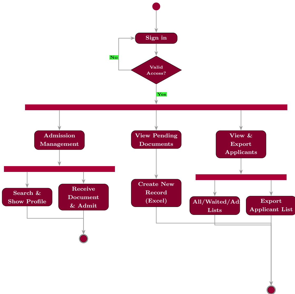
Figure 3.11: Activity Diagram of Registrar Office Management (UC-7.0)
