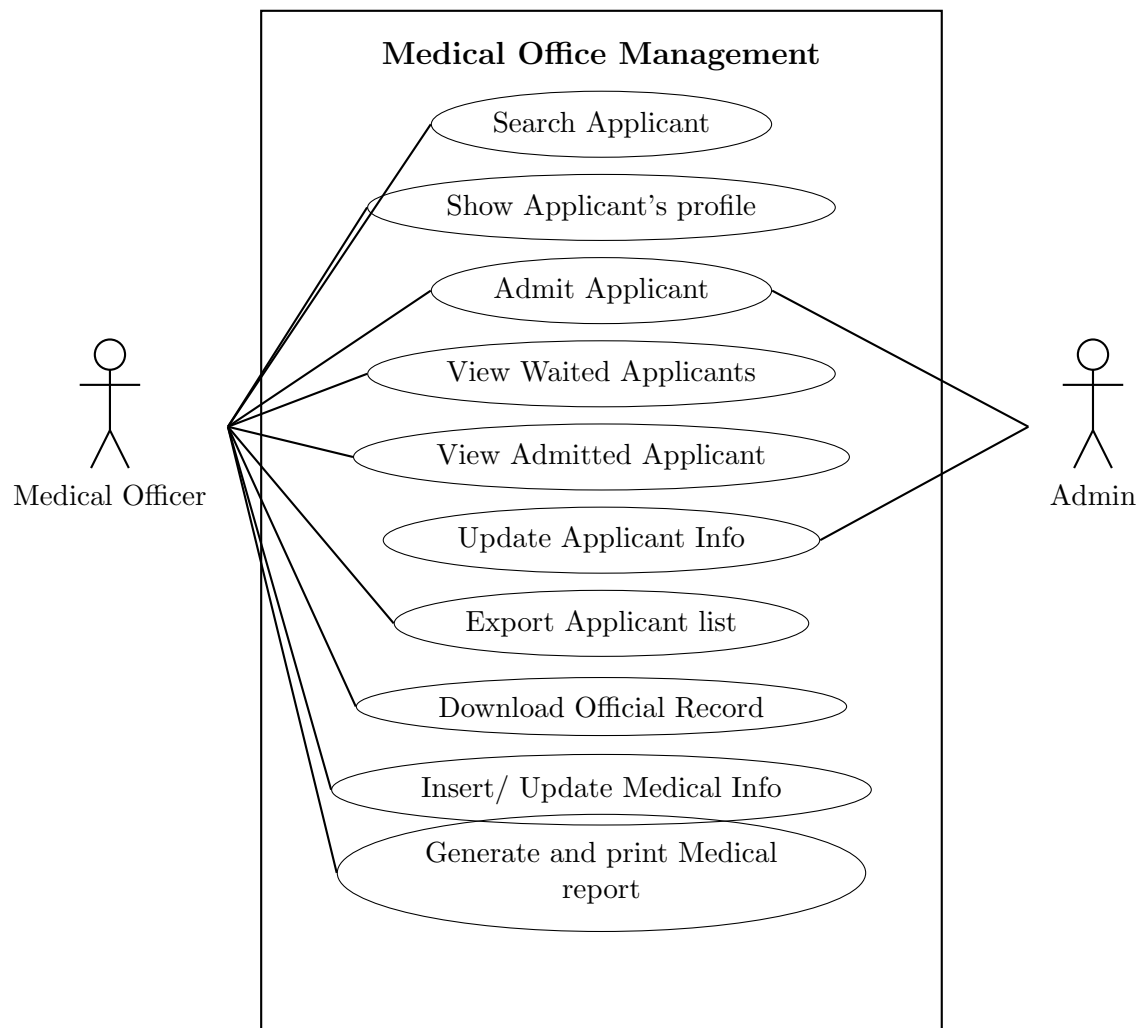
Figure 3.4: Use Case Diagram of Medical Office Management
