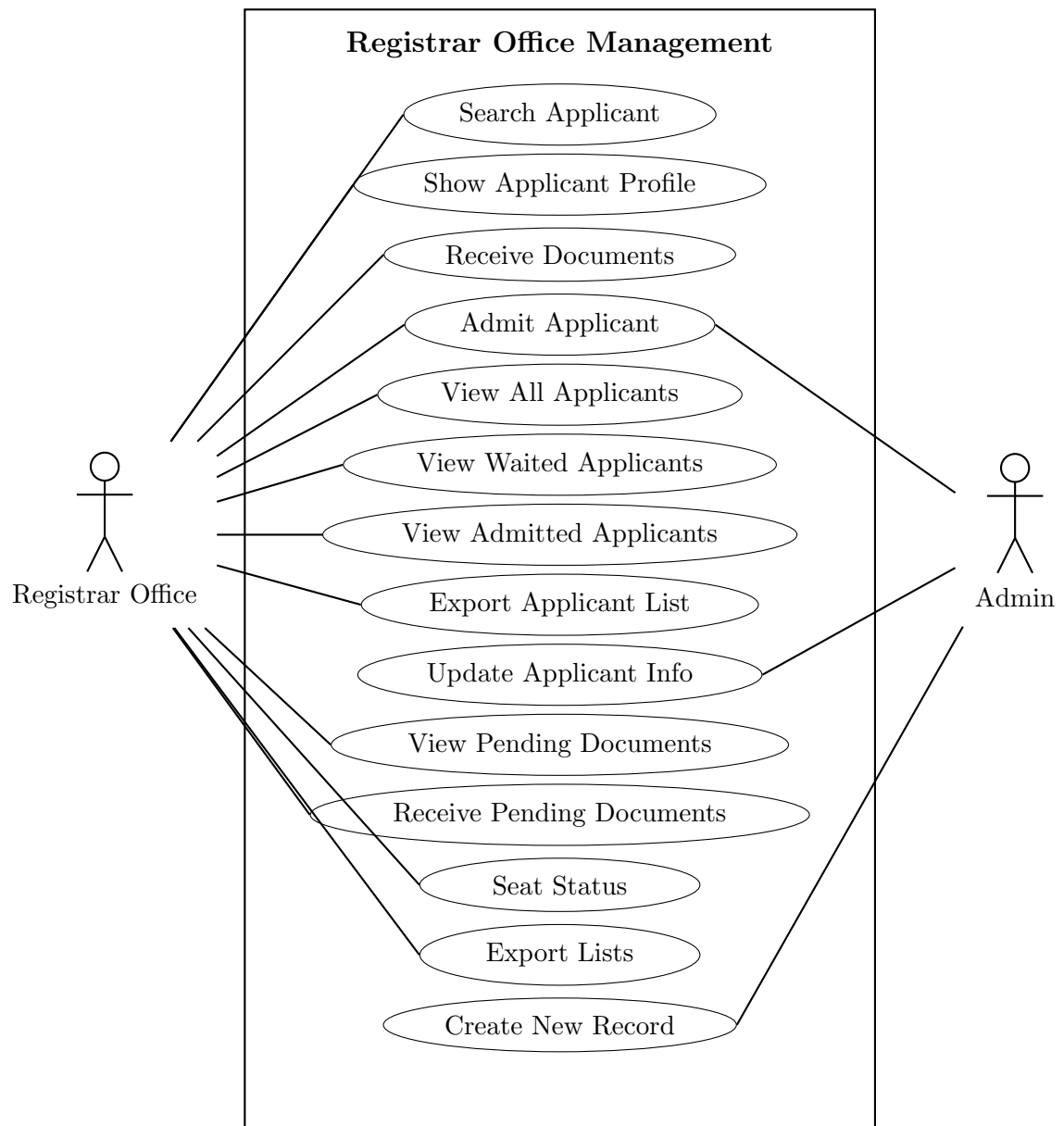
Figure 3.5: Use Case Diagram of Registrar Office Management
