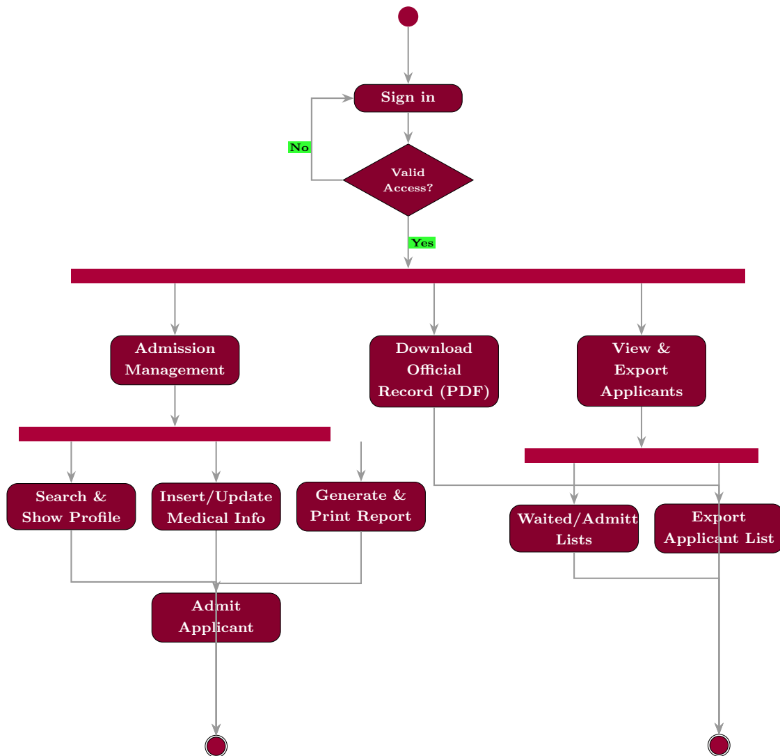
Figure 3.10: Activity Diagram of Medical Office Management (UC-4.0)
