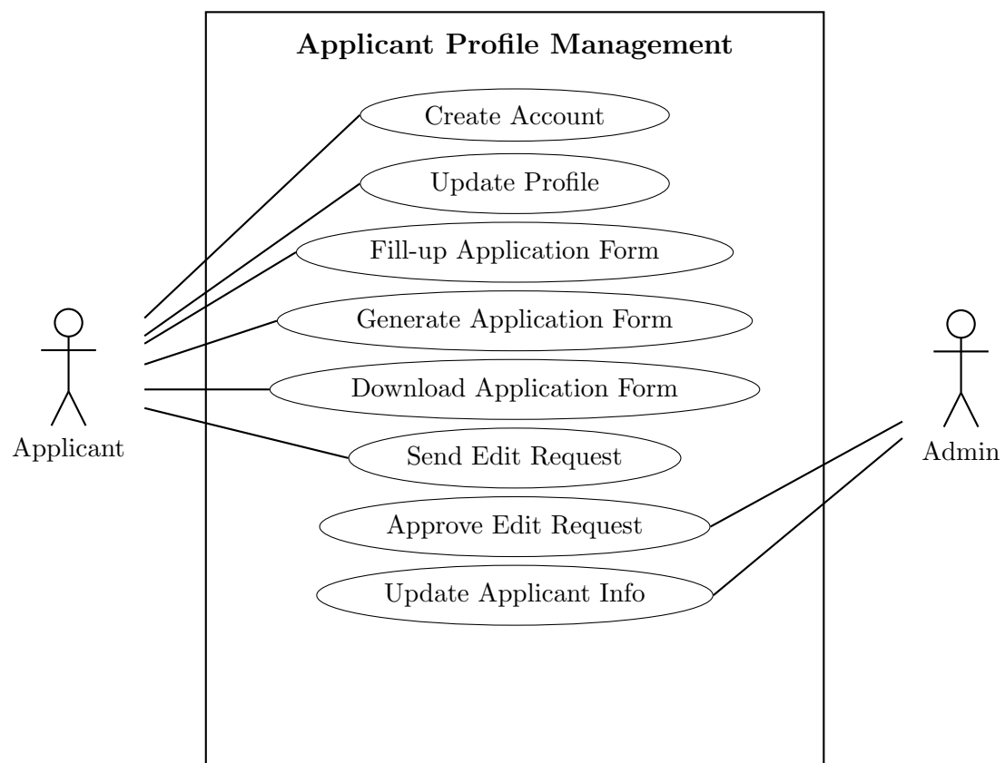
Figure 3.6: Use Case Diagram of Applicant Profile Management
