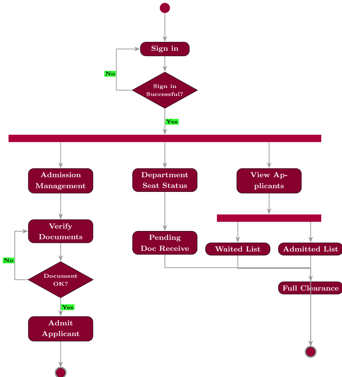
Figure 3.8: Activity Diagram of Dean Office Management (UC-5.0)
