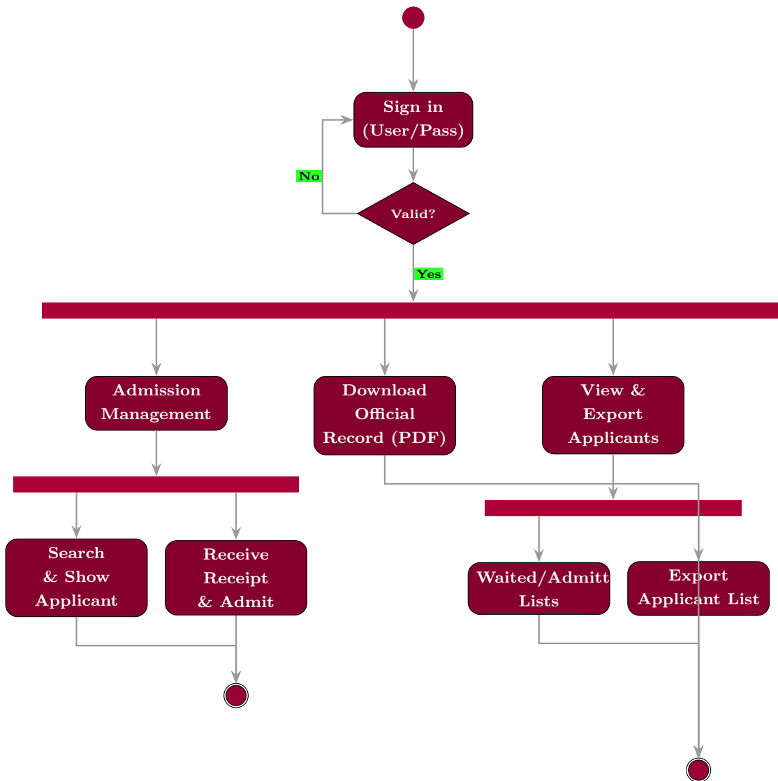
Figure 3.9: Activity Diagram of Hall Office Management (UC-6.0)
