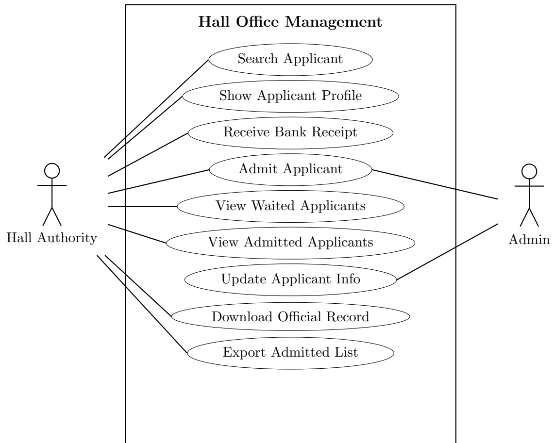
Figure 3.3: Use Case Diagram of Hall Office Management
