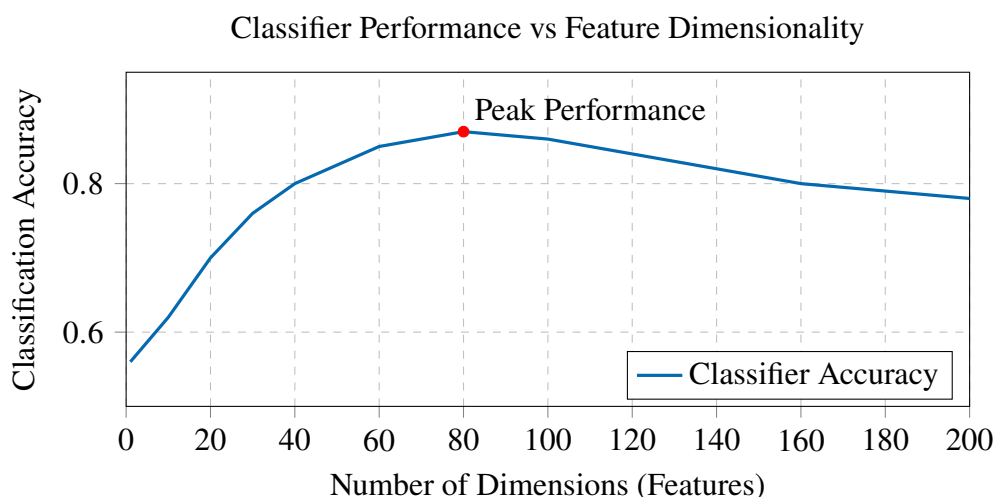
Figure 3.1: The trend of classifier performance with the change of dimension
