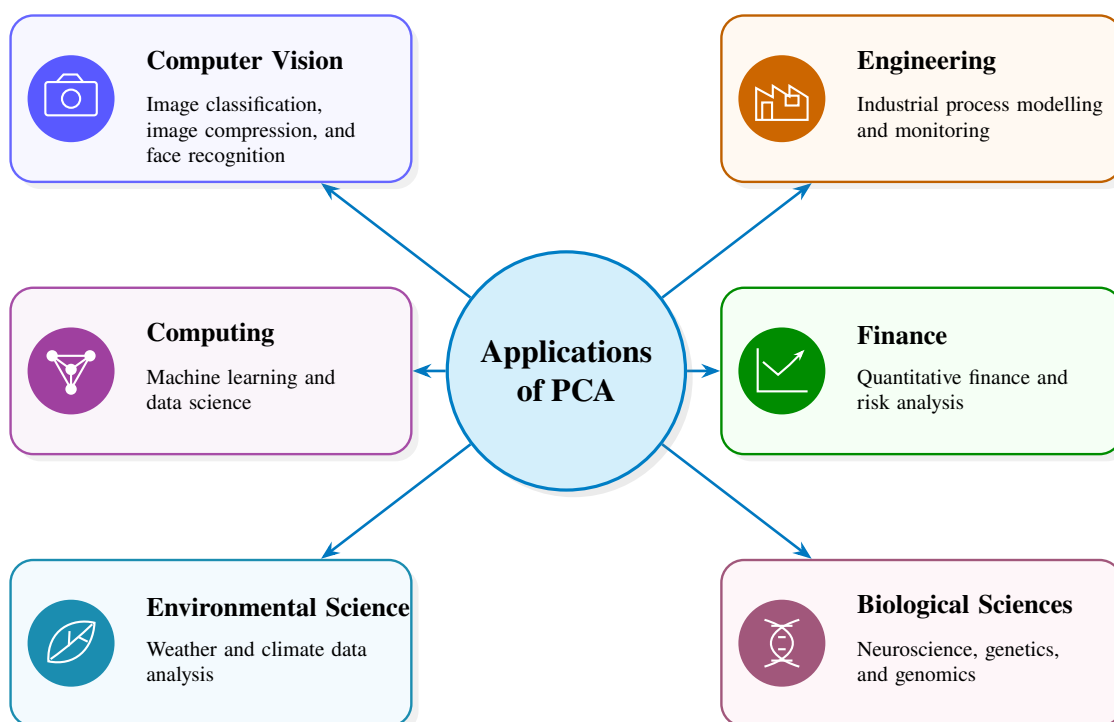
Figure 2.5: Scientific applications of Principal Component Analysis (PCA)
