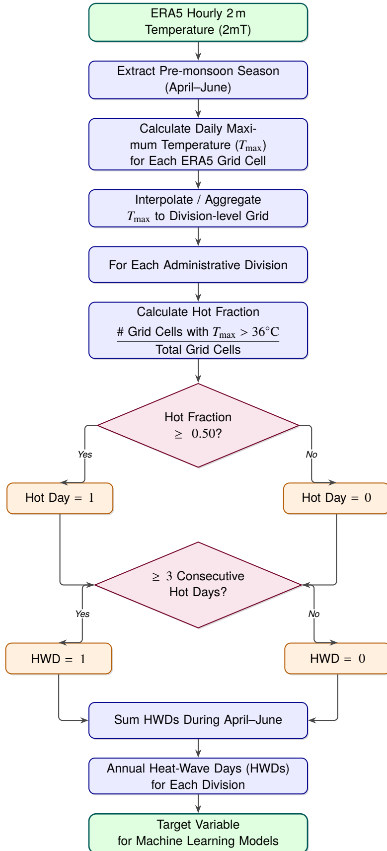
Figure 4.3: Flowchart for calculating annual Heat-Wave Days (HWDs) from ERA5 hourly 2 m temperature data
