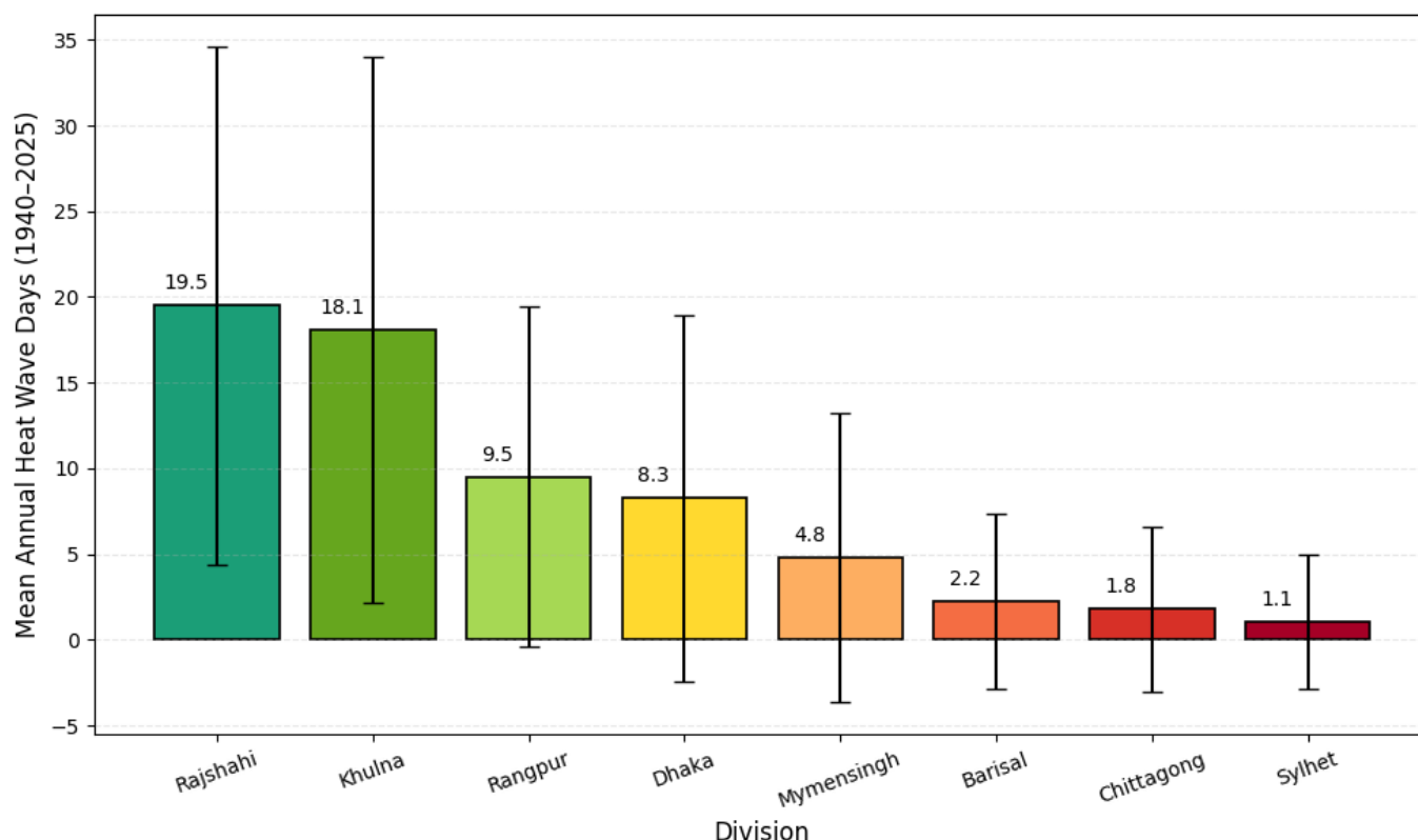
Figure 4.7: Spatial Distribution of Mean Annual Heat Wave Days Across Bangladesh's Divisions
