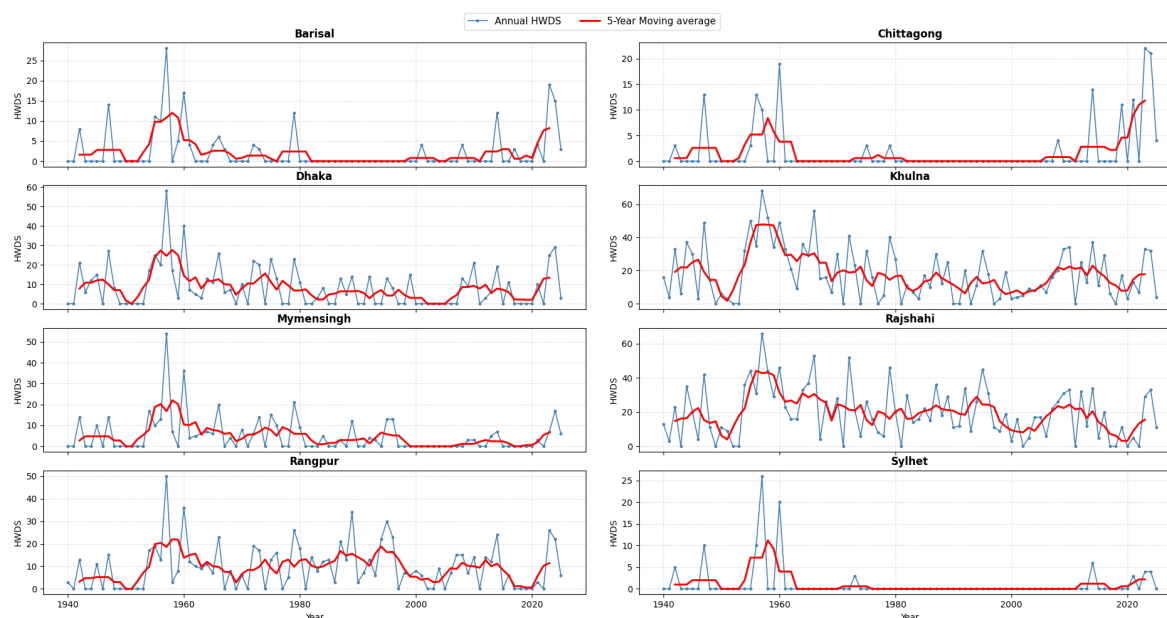
Figure 4.9: Annual heat wave days (HWDs) by division, 1940–2025, with 5-year moving average (red)
