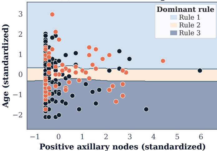
(a) Dominant rule regions
