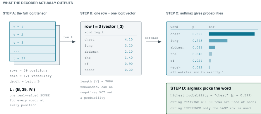
Figure 7: The decoder output explained in four steps: the full logit tensor, one row of it, the softmax that turns it into probabilities, and the argmax that selects a word.
