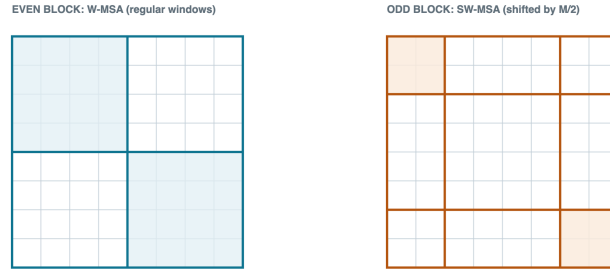
Figure 4: Regular versus shifted window partition, illustrated with M = 4 on an 8 \times 8 grid for legibility. The implementation uses M = 7 and s = 3 .
