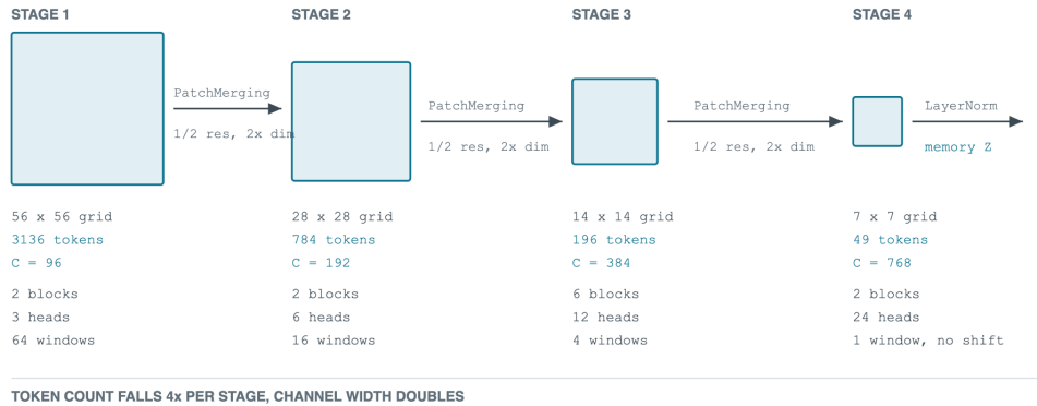
Figure 2: The four-stage hierarchy. Each PatchMerging step halves the grid resolution and doubles the channel width.
