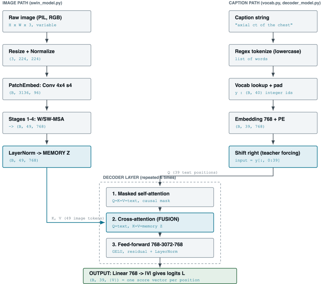
Figure 1: End-to-end architecture. The Swin encoder runs once per image and produces a fixed memory of 49 visual tokens. The decoder runs 6 identical layers, and only its cross-attention sub-layer reads that memory.
