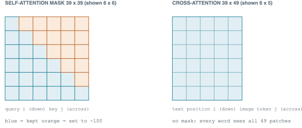
Figure 5: Self-attention is masked to a lower-triangular pattern; cross-attention is unmasked and fully dense.
