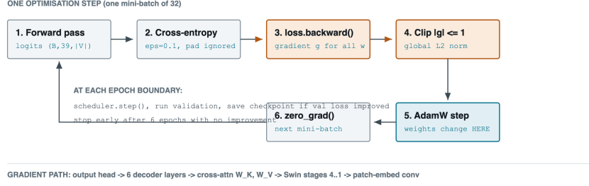
Figure 8: One optimisation step. The weights change only at step 5.
