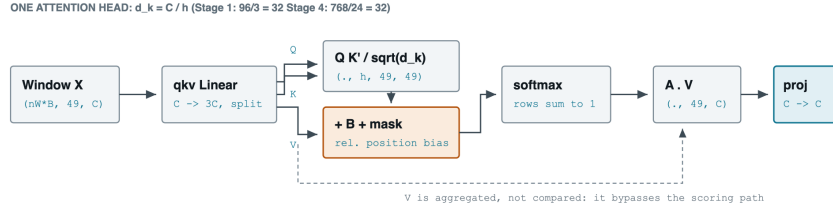
Figure 3: Data flow inside one attention head. The value matrix V is aggregated, not compared, so it bypasses the scoring path.
