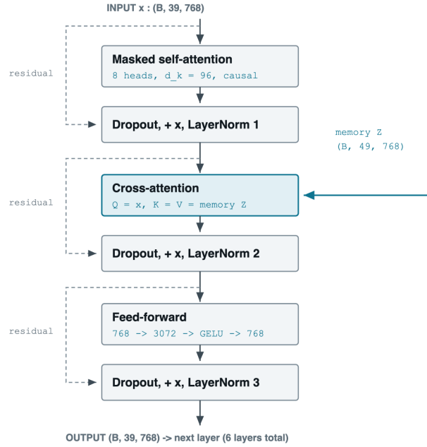
Figure 6: One decoder layer. Normalization is applied after the residual sum in each of the three sub-layers.
