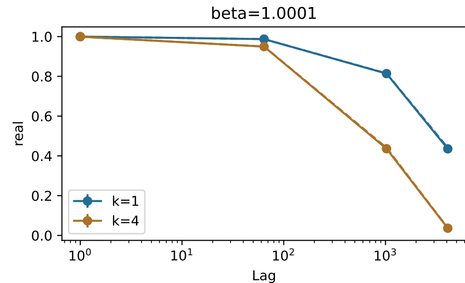
Lag correlations at T=1,000,000 | 64 independent seeds | approximate 95% CI
