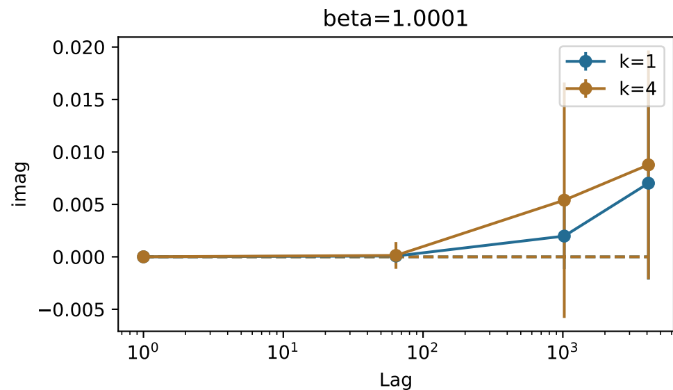
Lag correlations at T=1,000,000 | 64 independent seeds | approximate 95% CI
