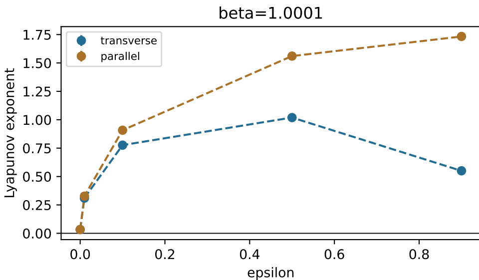
Additive coupling: theory (dashed) and 32-seed means | approximate 95% CI
