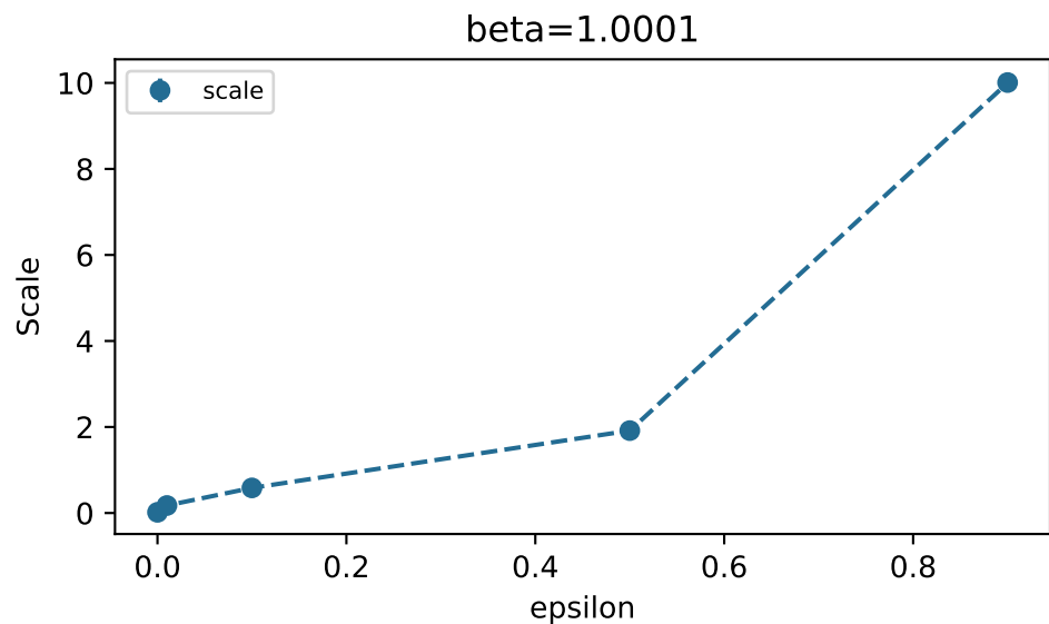
Additive coupling: theory (dashed) and 32-seed means | approximate 95% CI
