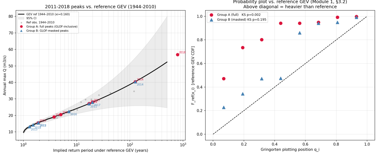
Figure 3: Left: 2011–2018 BAFU 2219 daily-maximum peaks on the reference GEV return-period curve (1944–2010). The 2018 GLOF-inclusive peak (crimson, \hat{T} \approx 789 yr) dominates; after masking it drops to \hat{T} \approx 1.5 yr (blue triangle). Right: probability plot (Module 1, §3.2; Passalacqua 2026). GLOF-inclusive lie far above the diagonal, driven by 2018. GLOF-masked lie systematically above the 1:1 line, indicating peaks slightly higher than the reference predicts.
