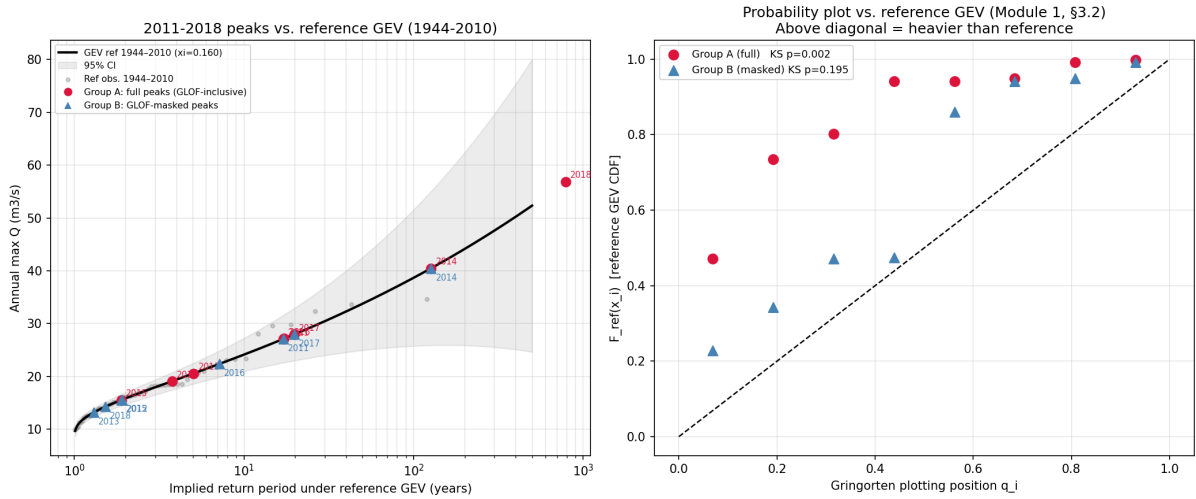
Figure 2: Left: 2011–2018 BAFU 2219 daily-maximum peaks on the reference GEV return-period curve (1944–2010). The 2018 GLOF-inclusive peak (crimson, \hat{T} \approx 789 yr) dominates; after masking it drops to \hat{T} \approx 1.5 yr (blue triangle). Right: probability plot (Module 1, §3.2). GLOF-inclusive lie far above the diagonal, driven by 2018. GLOF-masked lie systematically above the 1:1 line, indicating peaks slightly higher than the reference predicts.
