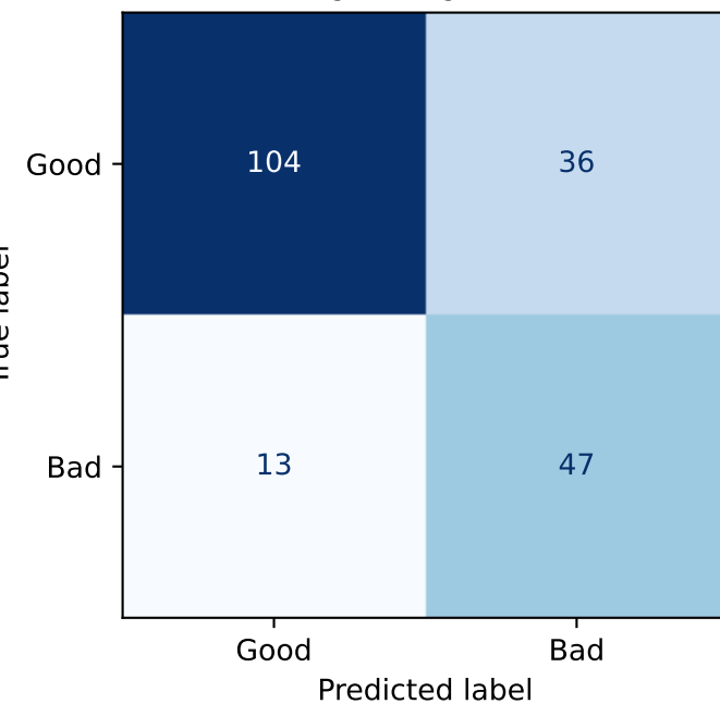
Logistic Regression
