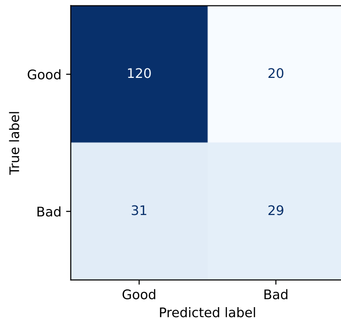
Random Forest
