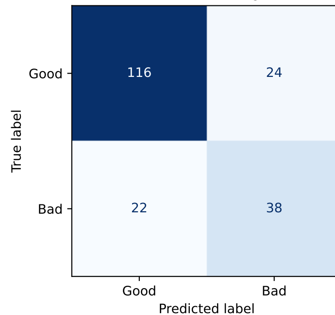
Gradient Boosting
