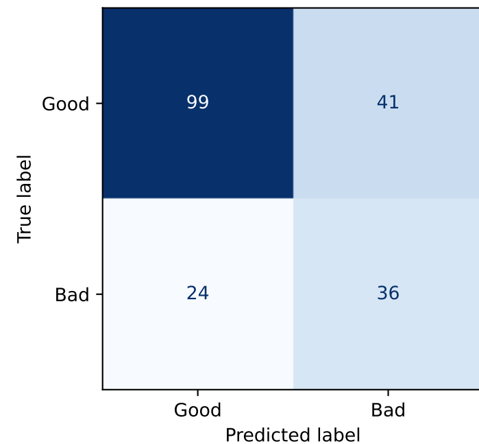
Decision Tree
