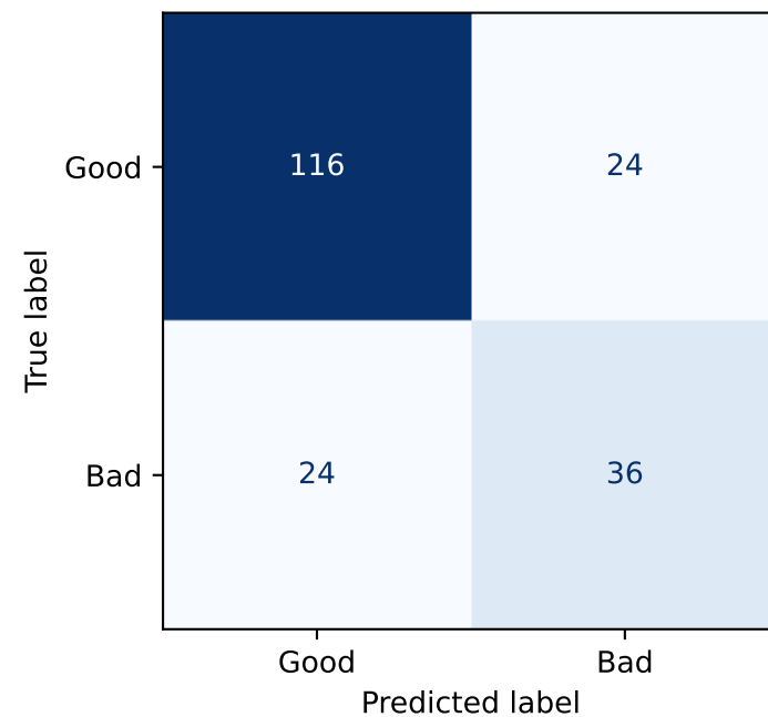
XGBoost
