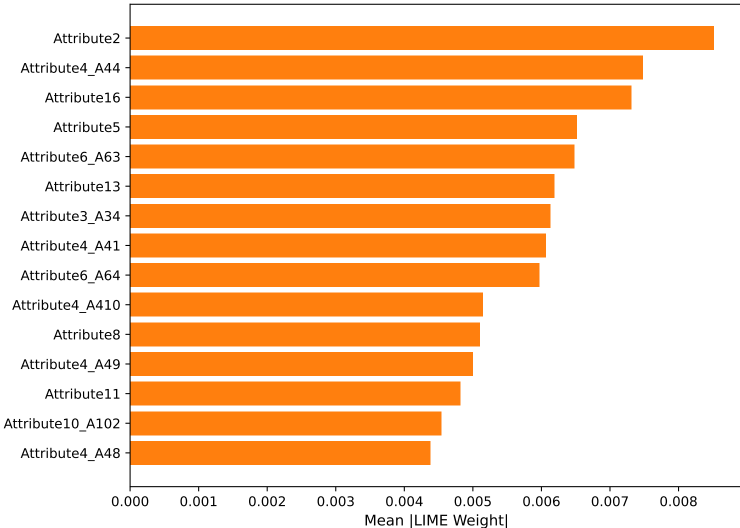
Top 15 Features — Gradient Boosting (LIME)
