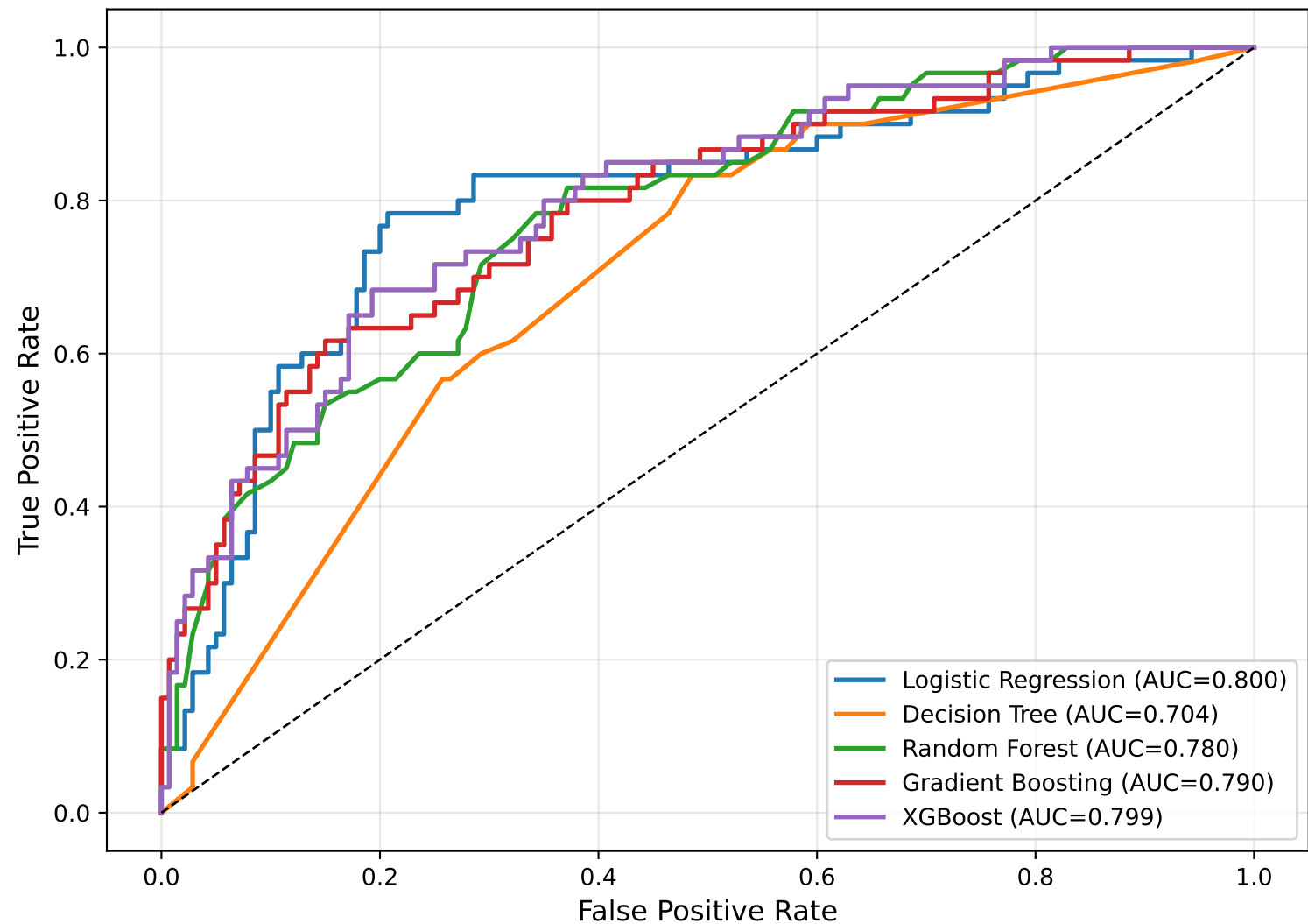
ROC Curves — All Models (Test Set)
