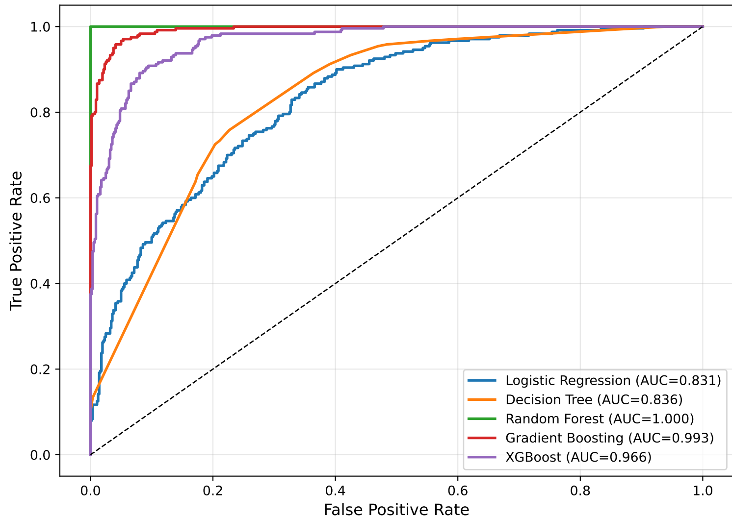
ROC Curves -- All Models (Train Set)
