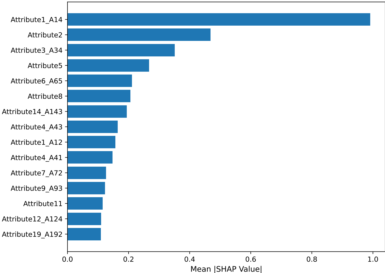
Top 15 Features — Gradient Boosting (SHAP)
