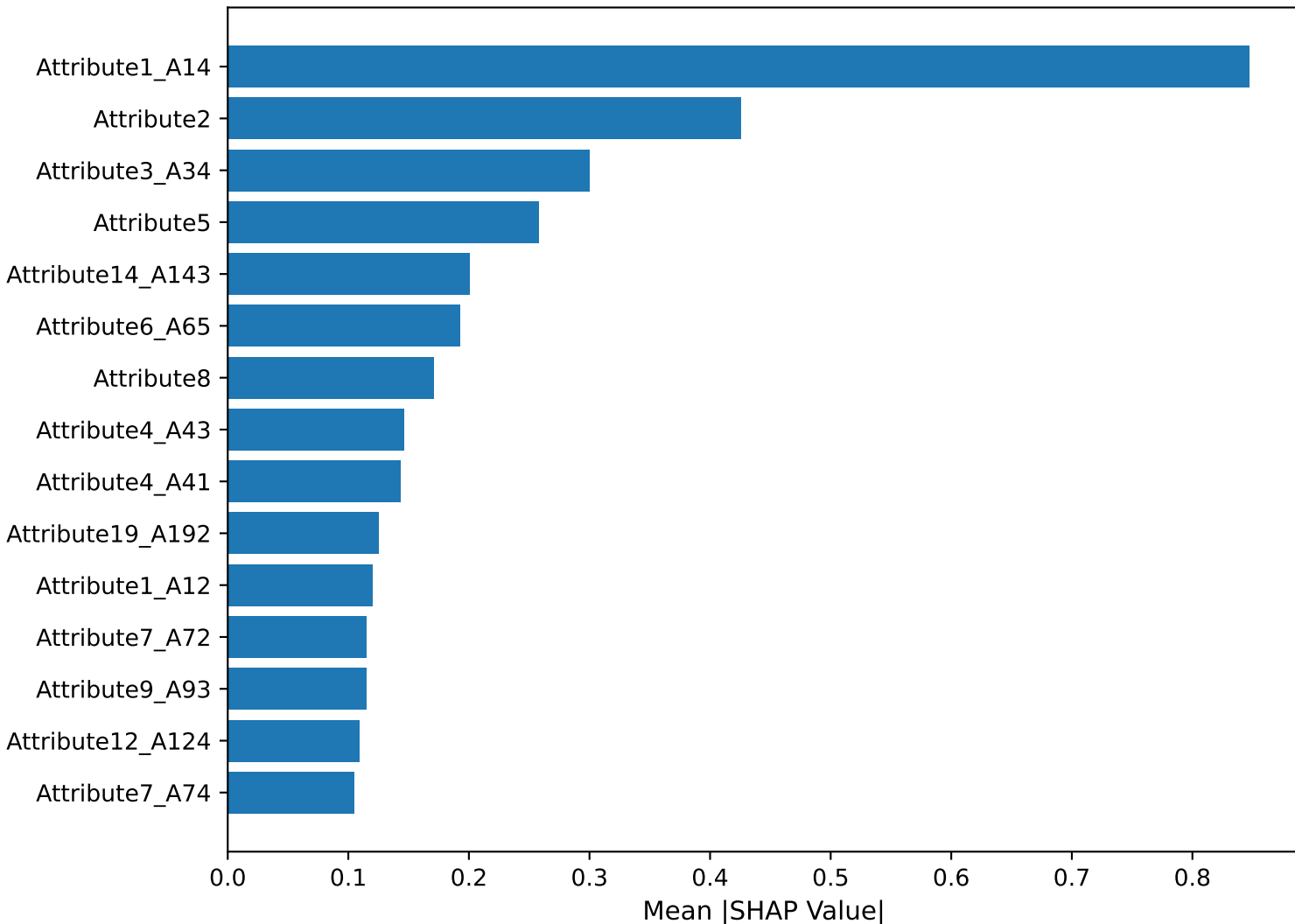
Top 15 Features — XGBoost (SHAP)
