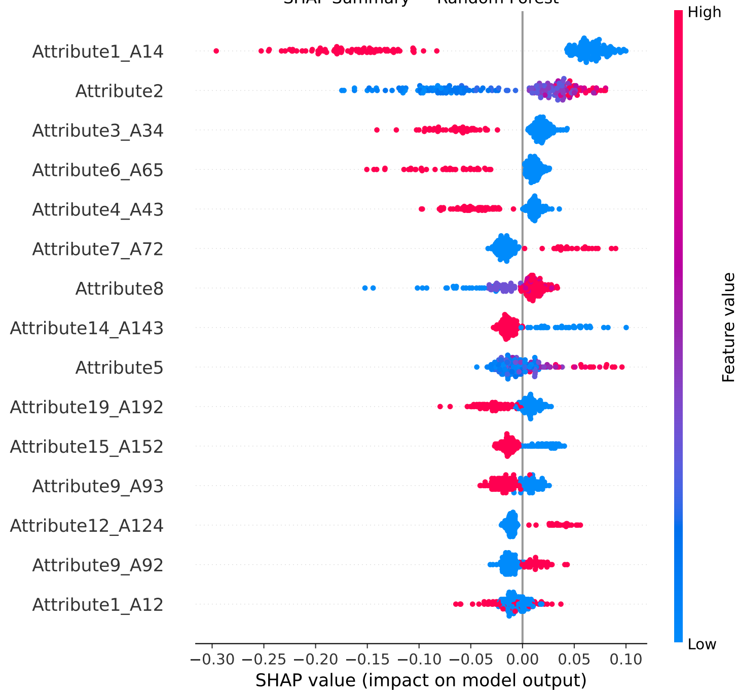
SHAP Summary — Random Forest
