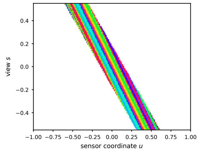
reflection E ( \div (1 - \alpha) ; view-dependent)
