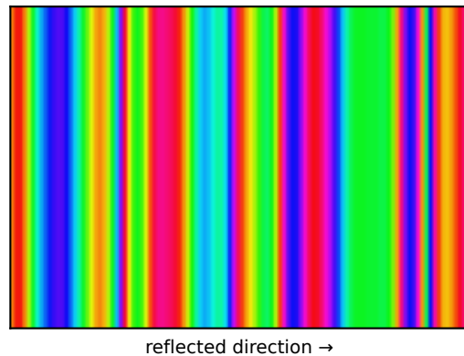
environment map E
