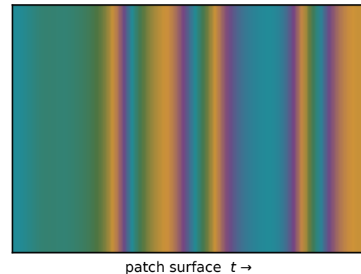
diffuse albedo D(t) (varies on patch)
