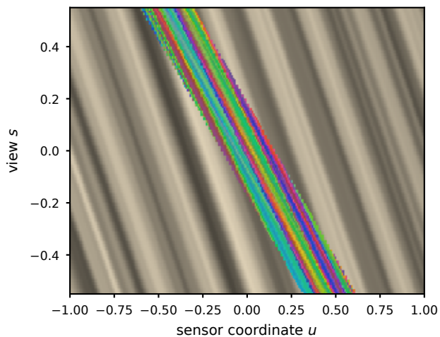
observed EPI O = \alpha D + (1 - \alpha)E
