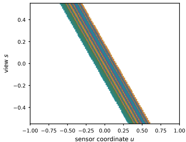
diffuse D ( \div \alpha ; constant along lines)
