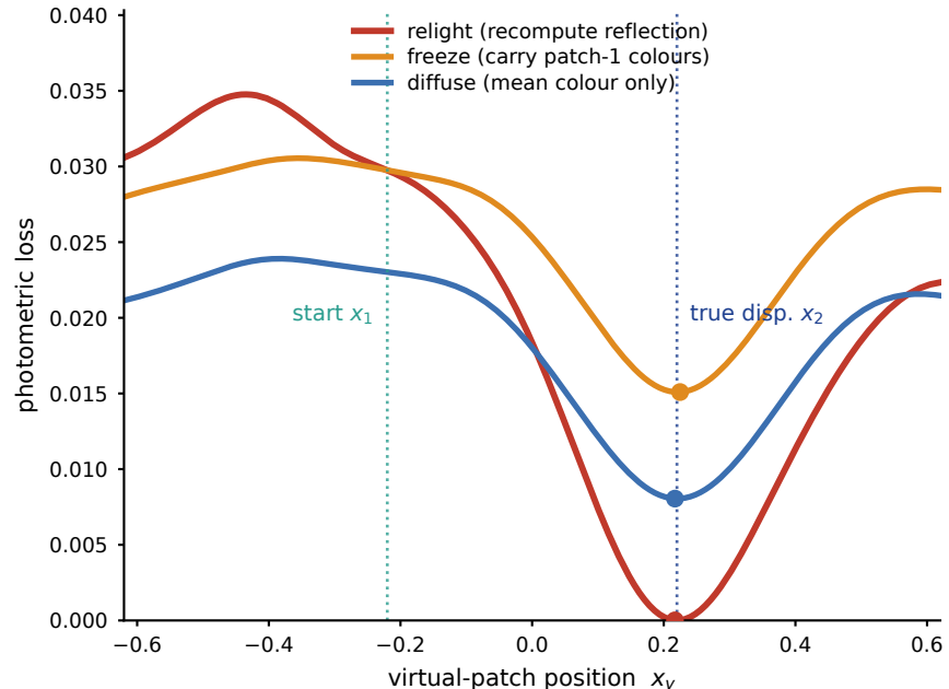
3 photometric loss vs candidate position
