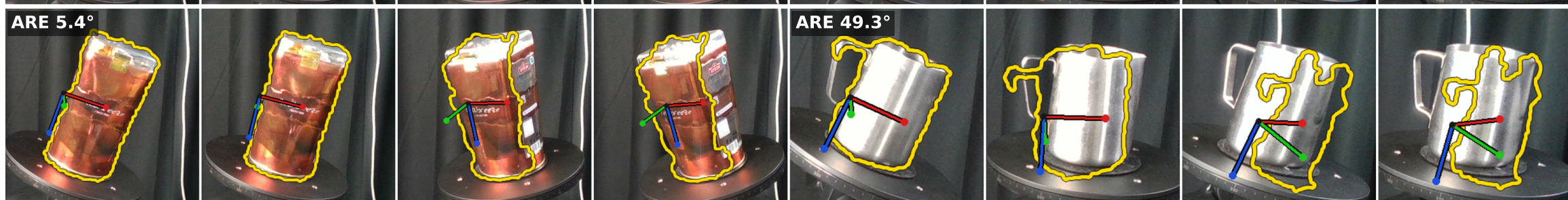
FoundationPose
