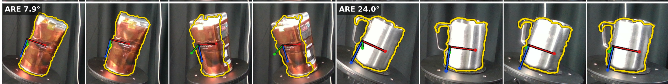
BundleSDF
