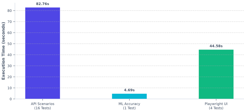
SachhAI Suite Runtimes by Category (s)
