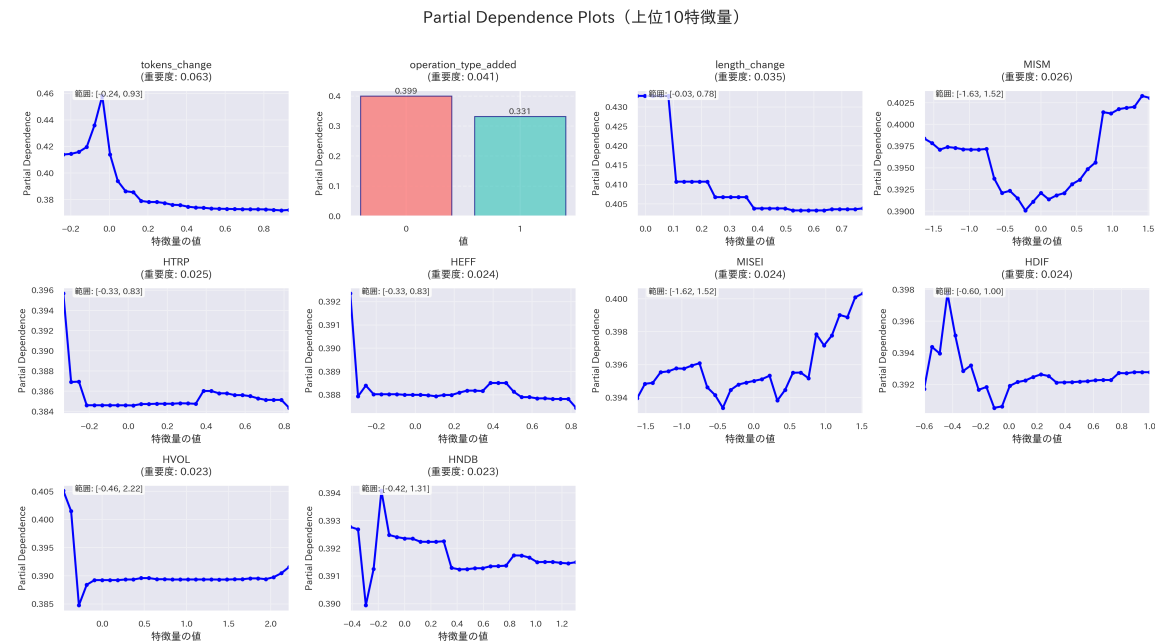
図8 ElasticsearchのPDP
