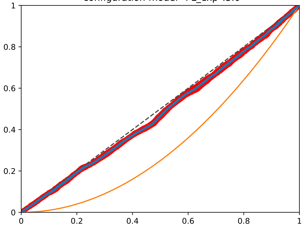
pagerank-20 vs. pagerank-70 Runs:5, graph size: 1000, all vertices configuration-model-"PL_exp":3.0
