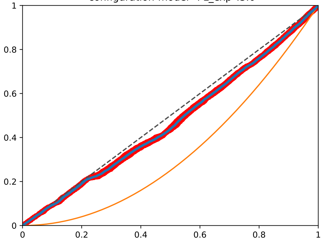
pagerank-40 vs. pagerank-90 Runs:5, graph size: 1000, all vertices configuration-model-"PL_exp":3.0
