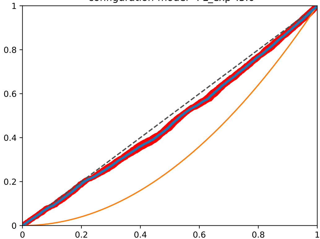
pagerank-20 vs. pagerank-80 Runs:5, graph size: 1000, all vertices configuration-model-"PL_exp":3.0
