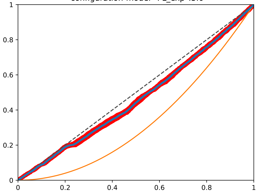
pagerank-20 vs. pagerank-90 Runs:5, graph size: 1000, all vertices configuration-model-"PL_exp":3.0
