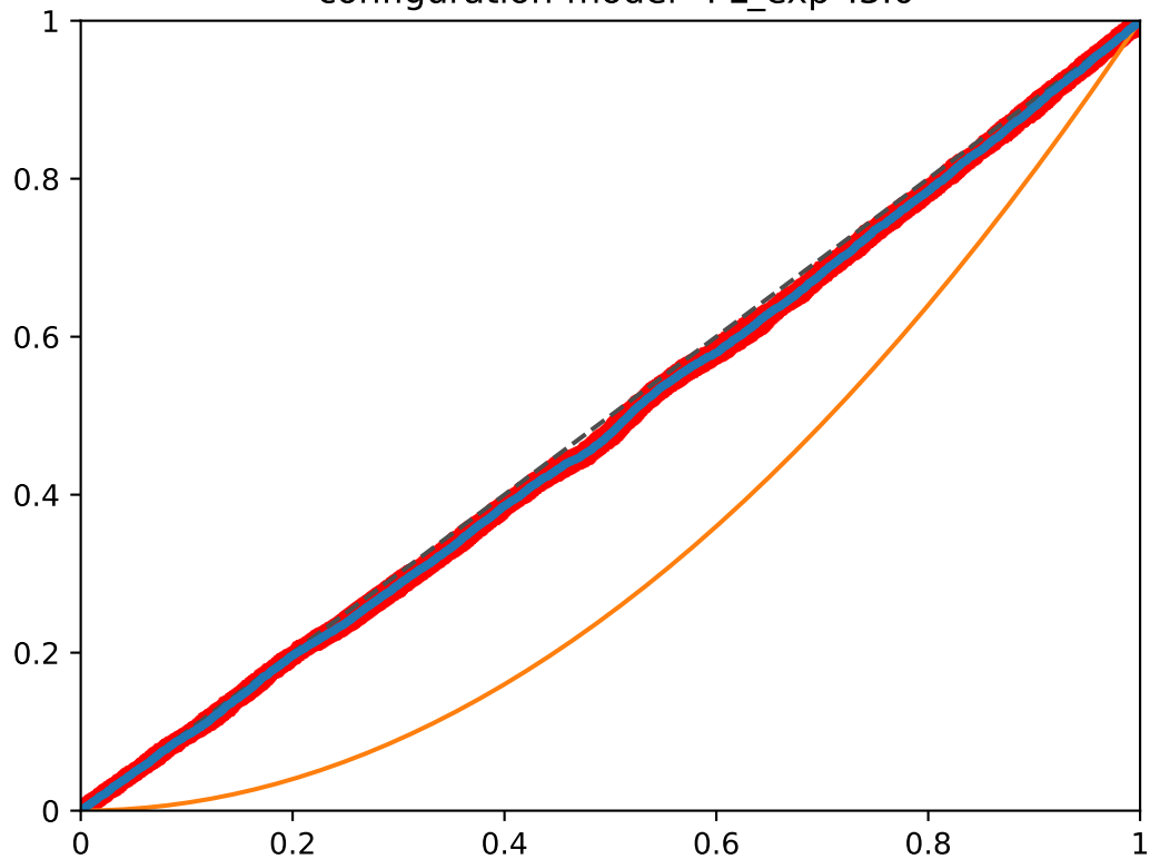
pagerank-30 vs. pagerank-60 Runs:5, graph size: 1000, all vertices configuration-model-"PL_exp":3.0
