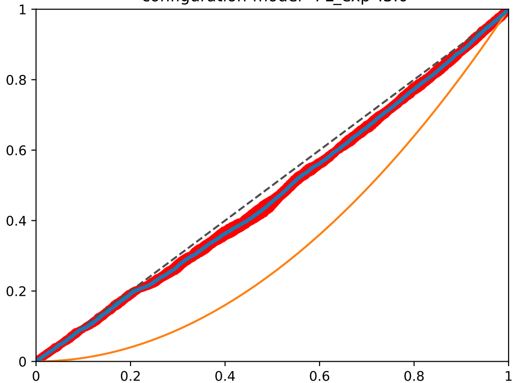
pagerank-30 vs. pagerank-80 Runs:5, graph size: 1000, all vertices configuration-model-"PL_exp":3.0
