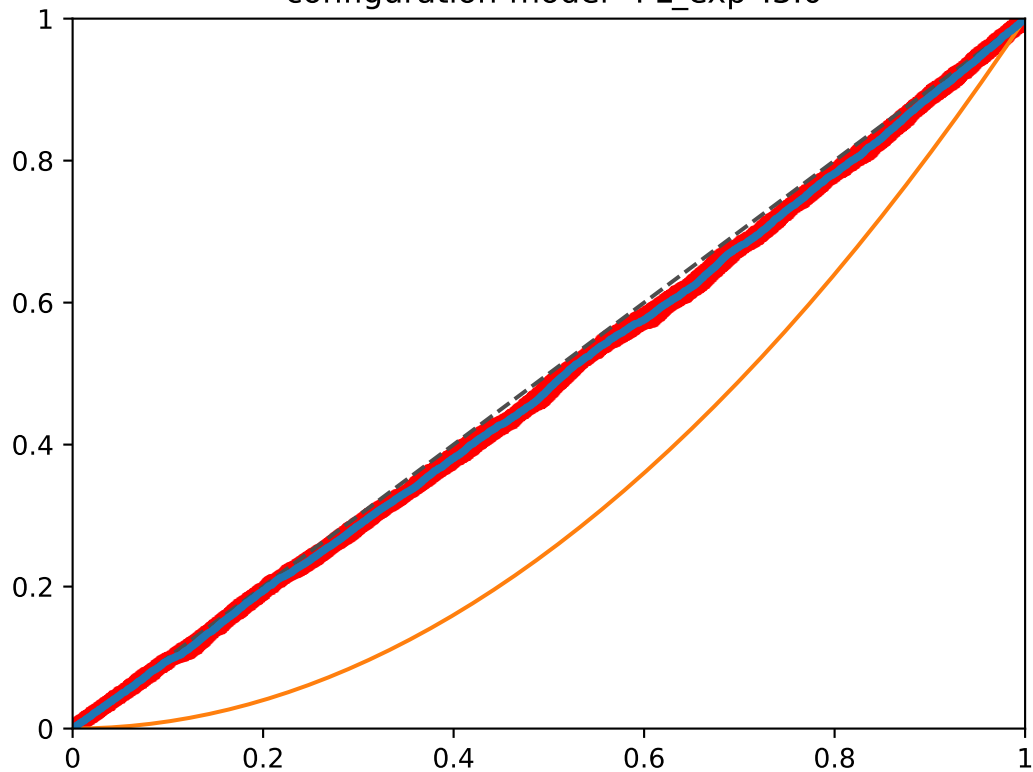
pagerank-20 vs. pagerank-60 Runs:5, graph size: 1000, all vertices configuration-model-"PL_exp":3.0
