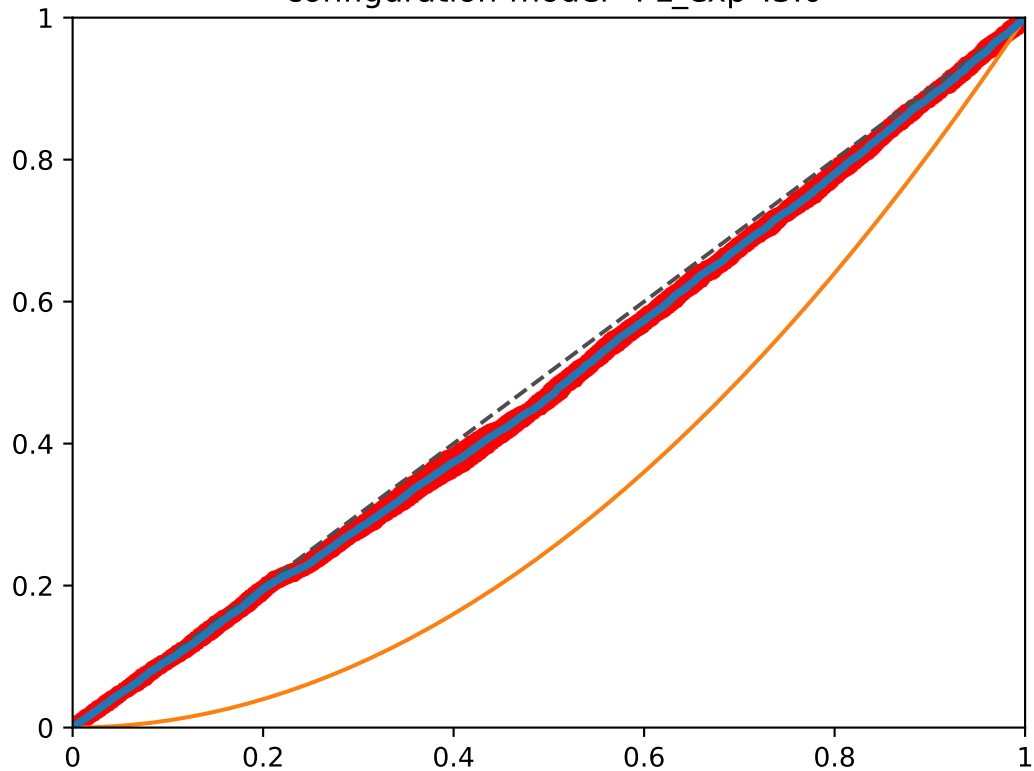
pagerank-50 vs. pagerank-80 Runs:5, graph size: 1000, all vertices configuration-model-"PL_exp":3.0
