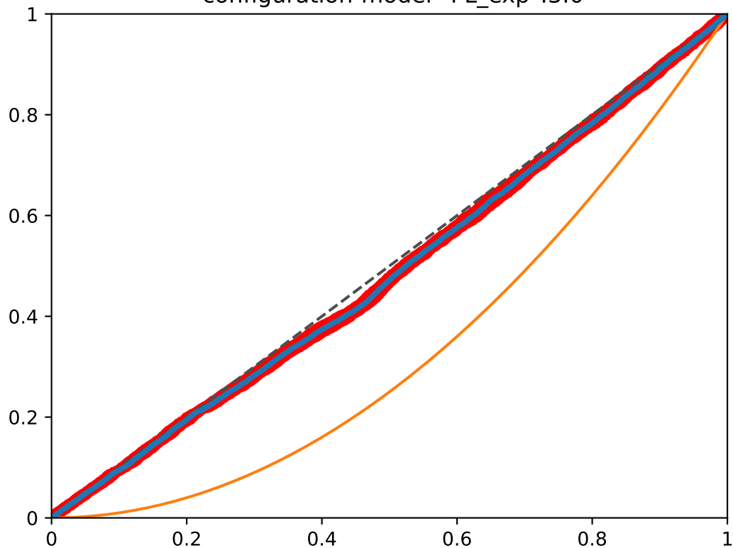
pagerank-40 vs. pagerank-70 Runs:5, graph size: 1000, all vertices configuration-model-"PL_exp":3.0
