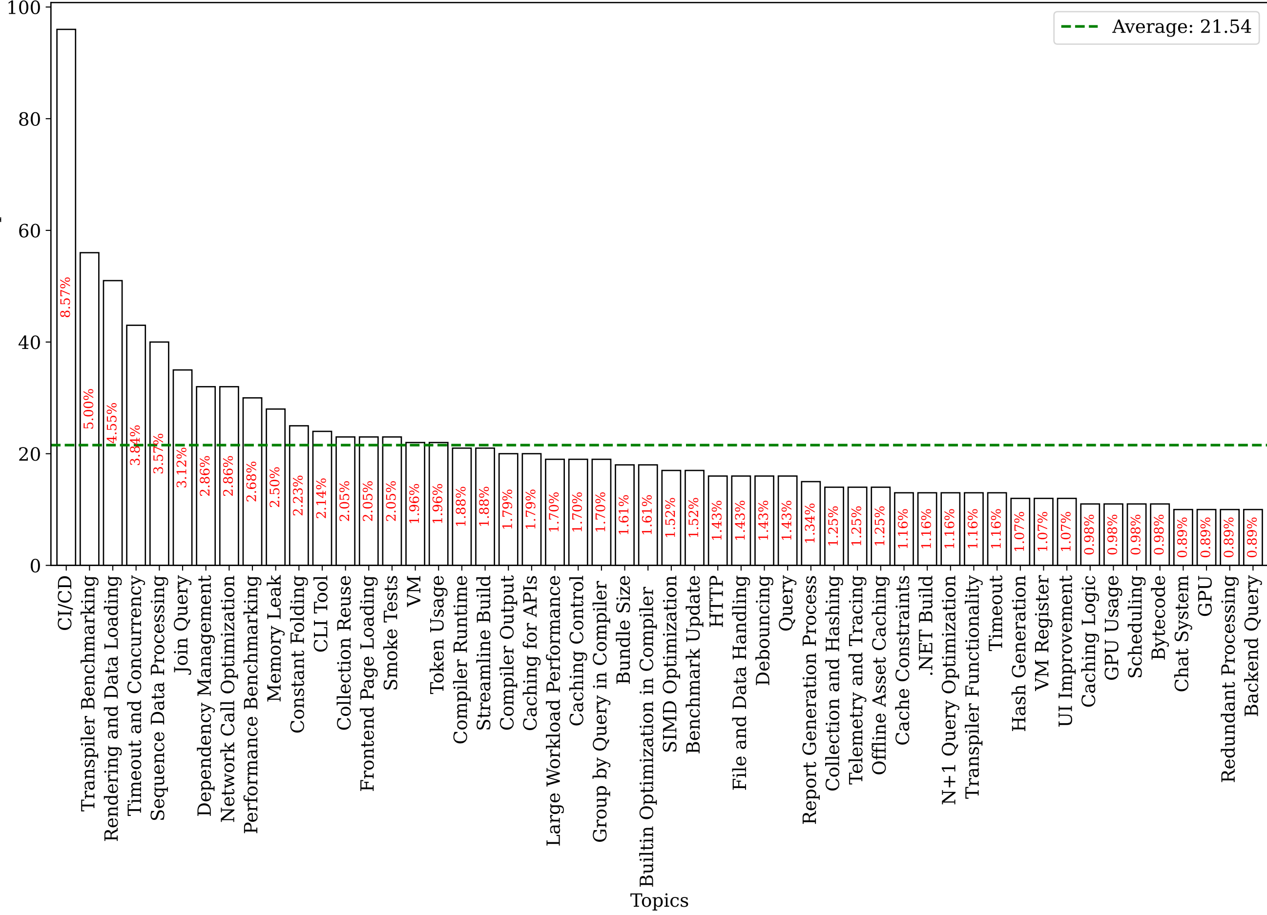
Number of Pull Requests
