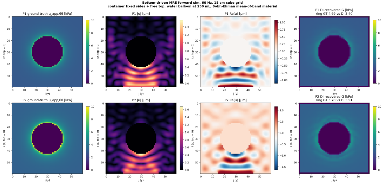
Figure 4: Bottom-plate driver run. Rows: P1 (top), P2 (bottom). Columns: ground-truth \mu_{\text{app},90} , wave amplitude |u| in \mu\text{m} , real part \Re(u) , DI-recovered G (with 3 \times 3 \times 3 median). Peak |u| = 1.57 \mu\text{m} (P1), 1.68 \mu\text{m} (P2) from a 1 \mu\text{m} driver amplitude. Ring stiffness (12 mm shell): DI recovers 3.40 kPa (P1) and 3.91 kPa (P2), vs ground truth 4.69 / 5.70 kPa — DI under-reads by 27–31%.
