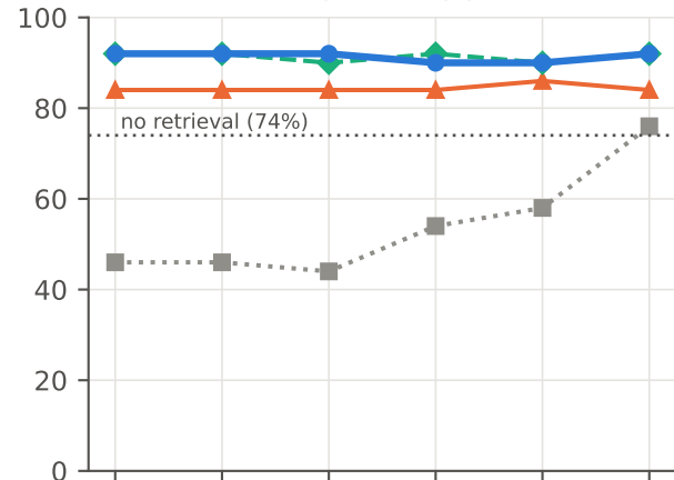
MS-MARCO
