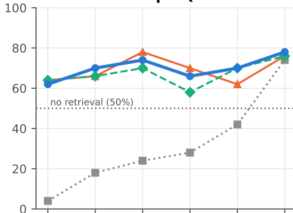
HotpotQA
