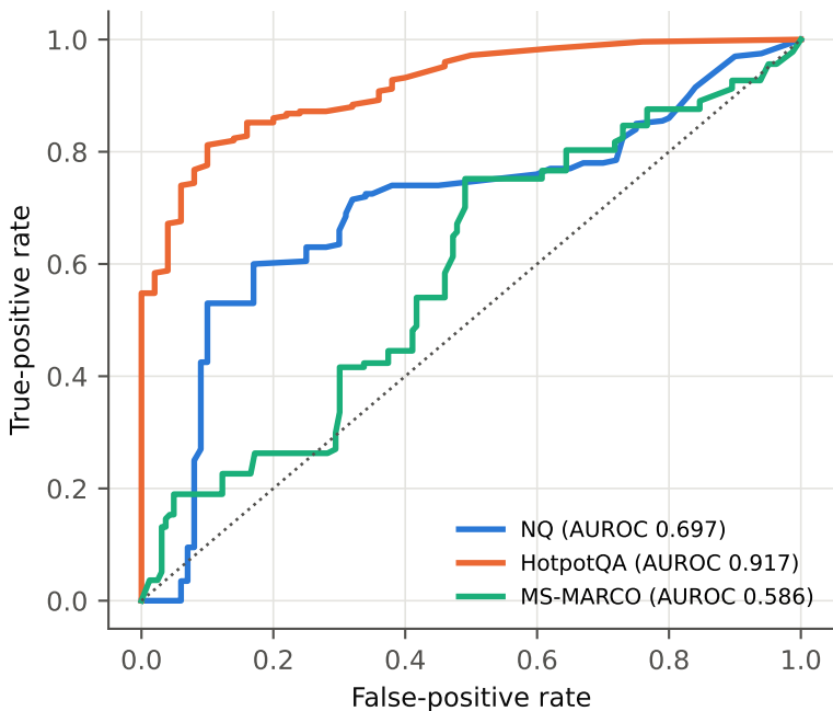
Pipeline risk score as a poisoning detector
