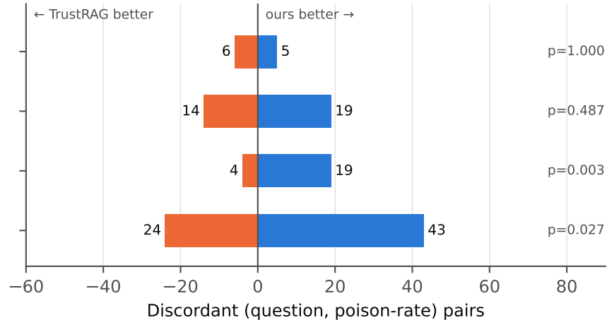
Successful attacks (ASR)
