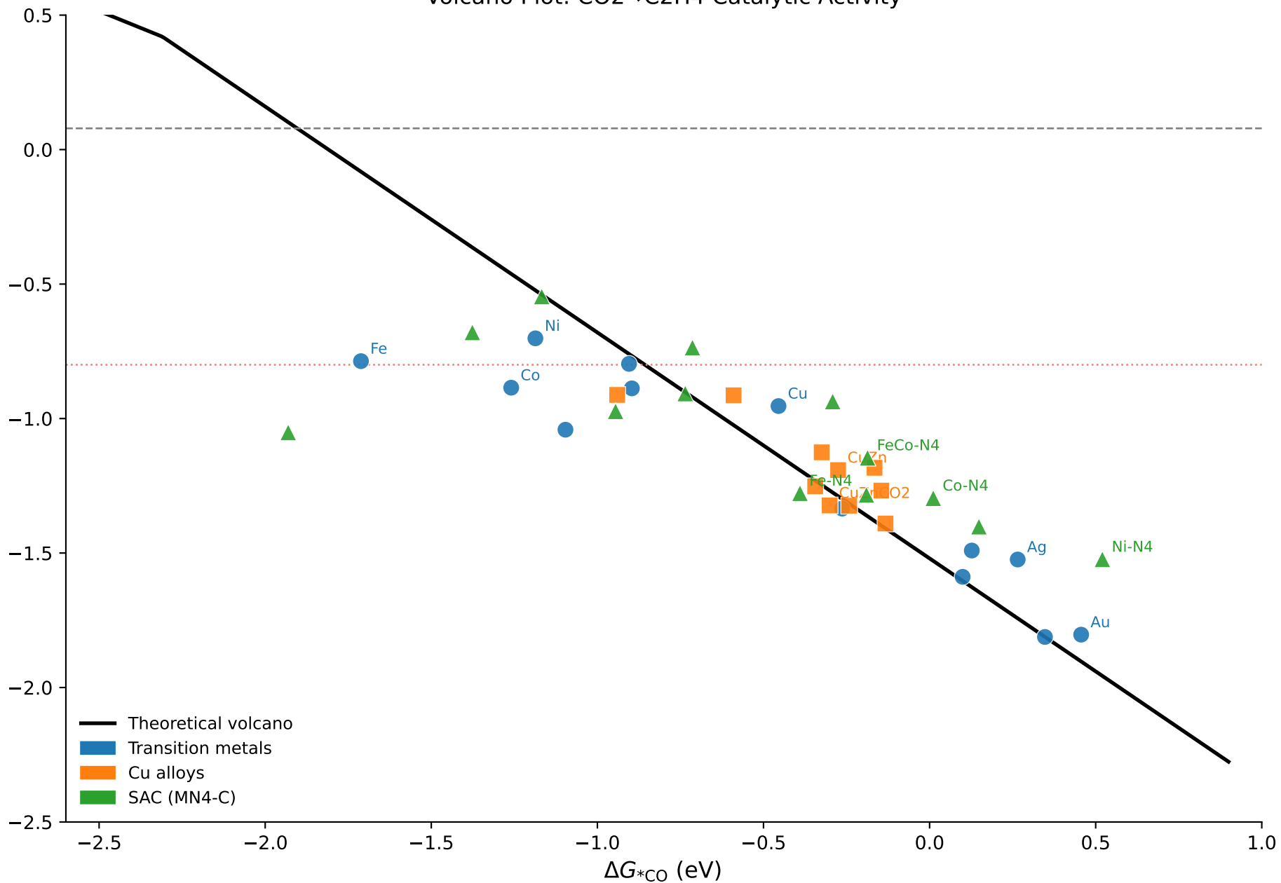
Volcano Plot: CO 2 →C 2 H 4 Catalytic Activity
