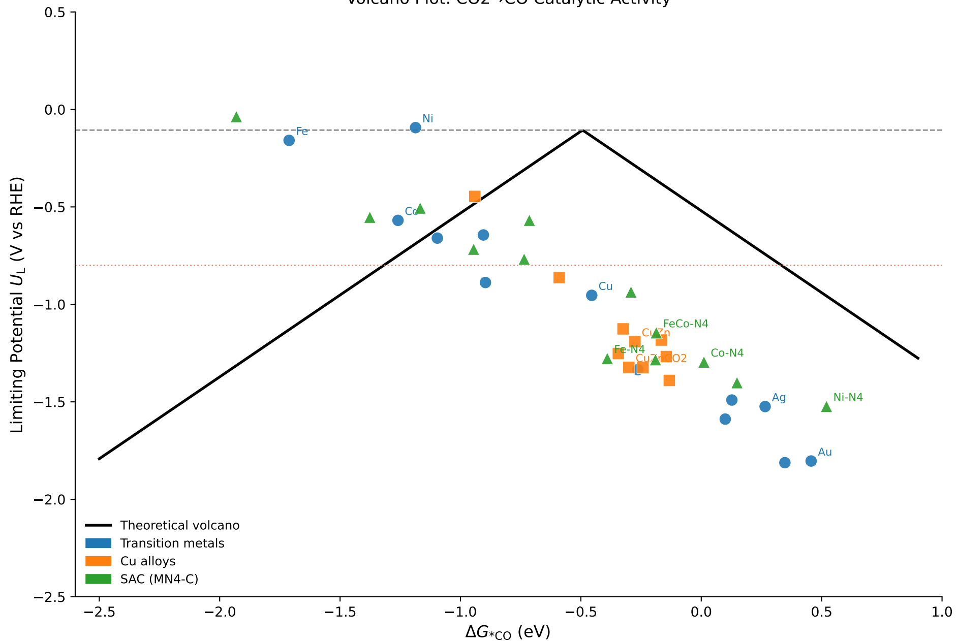
Volcano Plot: CO 2 →CO Catalytic Activity
