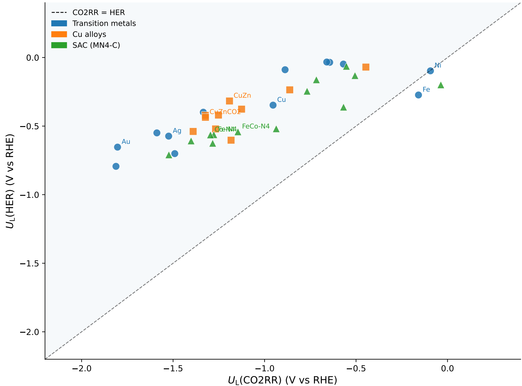
CO2RR vs HER Selectivity Map
