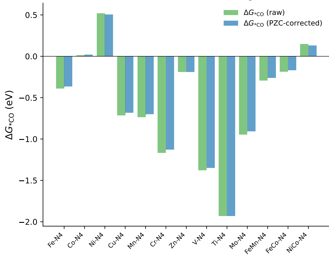
PZC Correction Effect on SAC CO* Binding ( U = -0.8 V)
