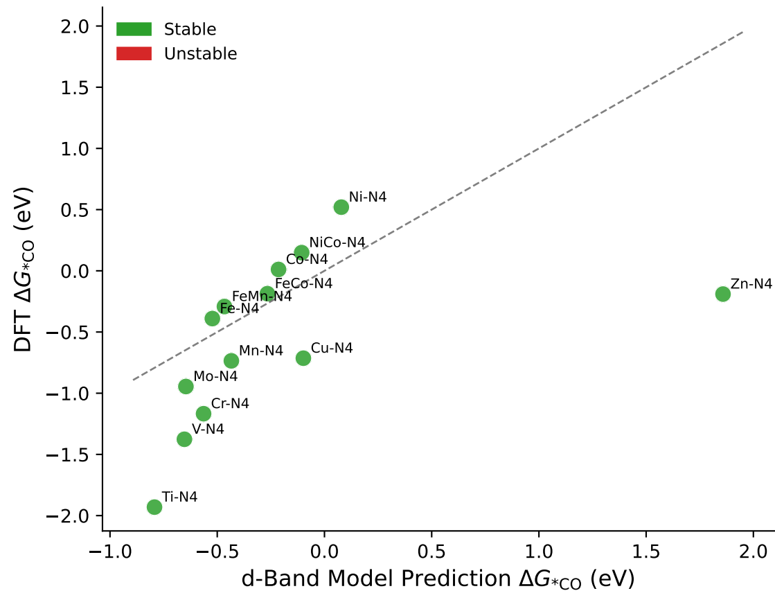
d-Band Centre Model vs DFT (SAC)
