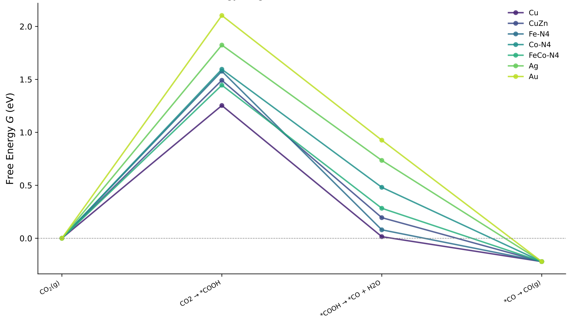
Free Energy Diagram: \text{CO}_2 \rightarrow \text{CO} at U = 0 \text{ V} vs RHE
