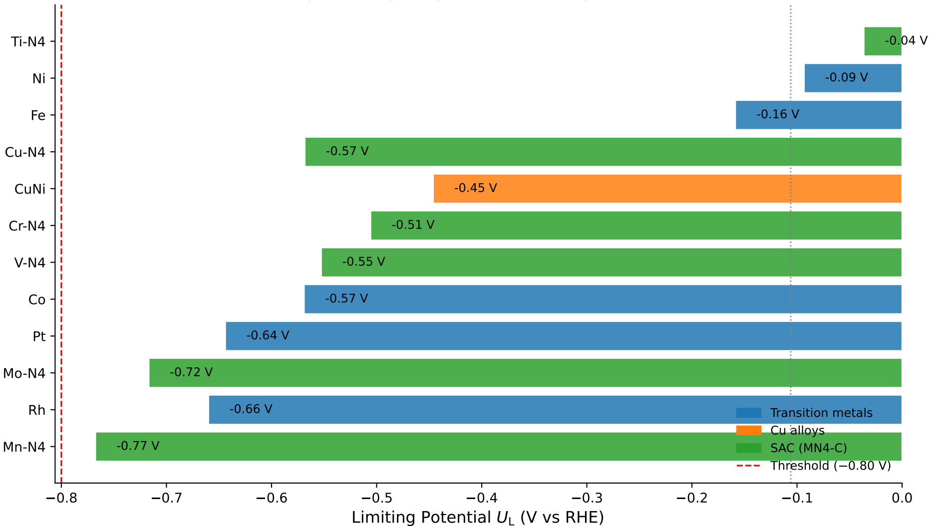
Top 12 Catalysts by CO 2 →CO Limiting Potential
