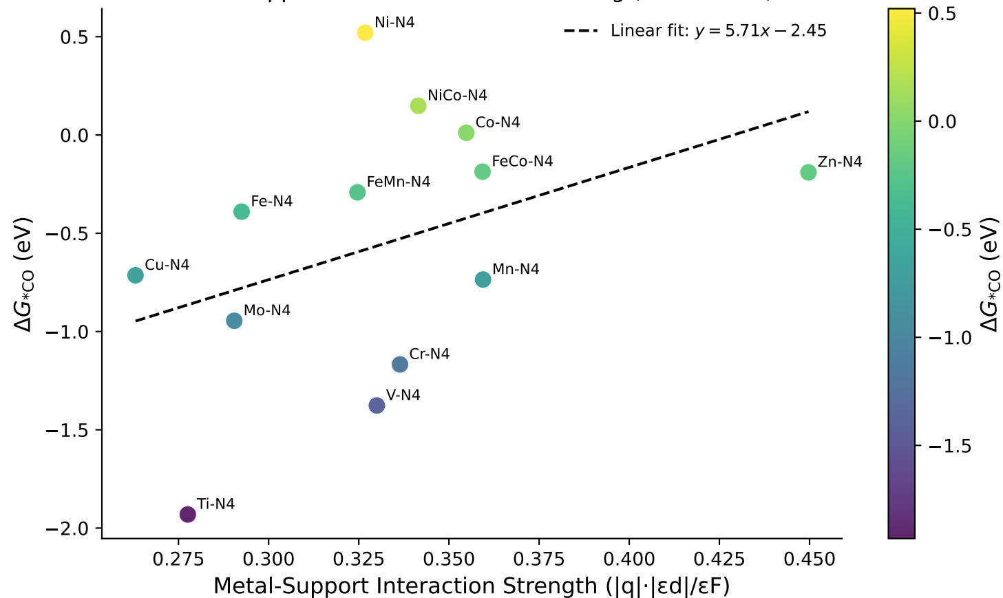
Metal-Support Interaction vs CO* Binding (SAC MN4-C)
