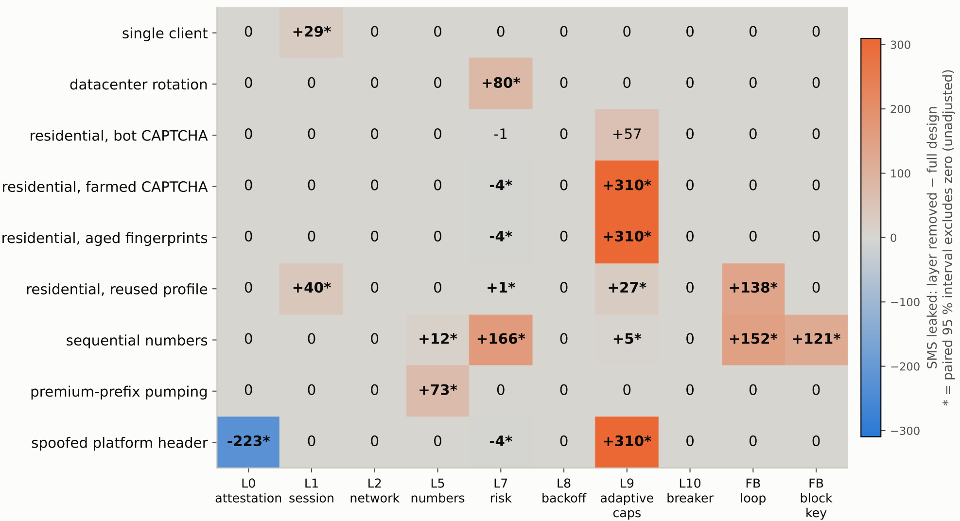
layer removed (one at a time; conditional effects in this pipeline, they do not add up)
