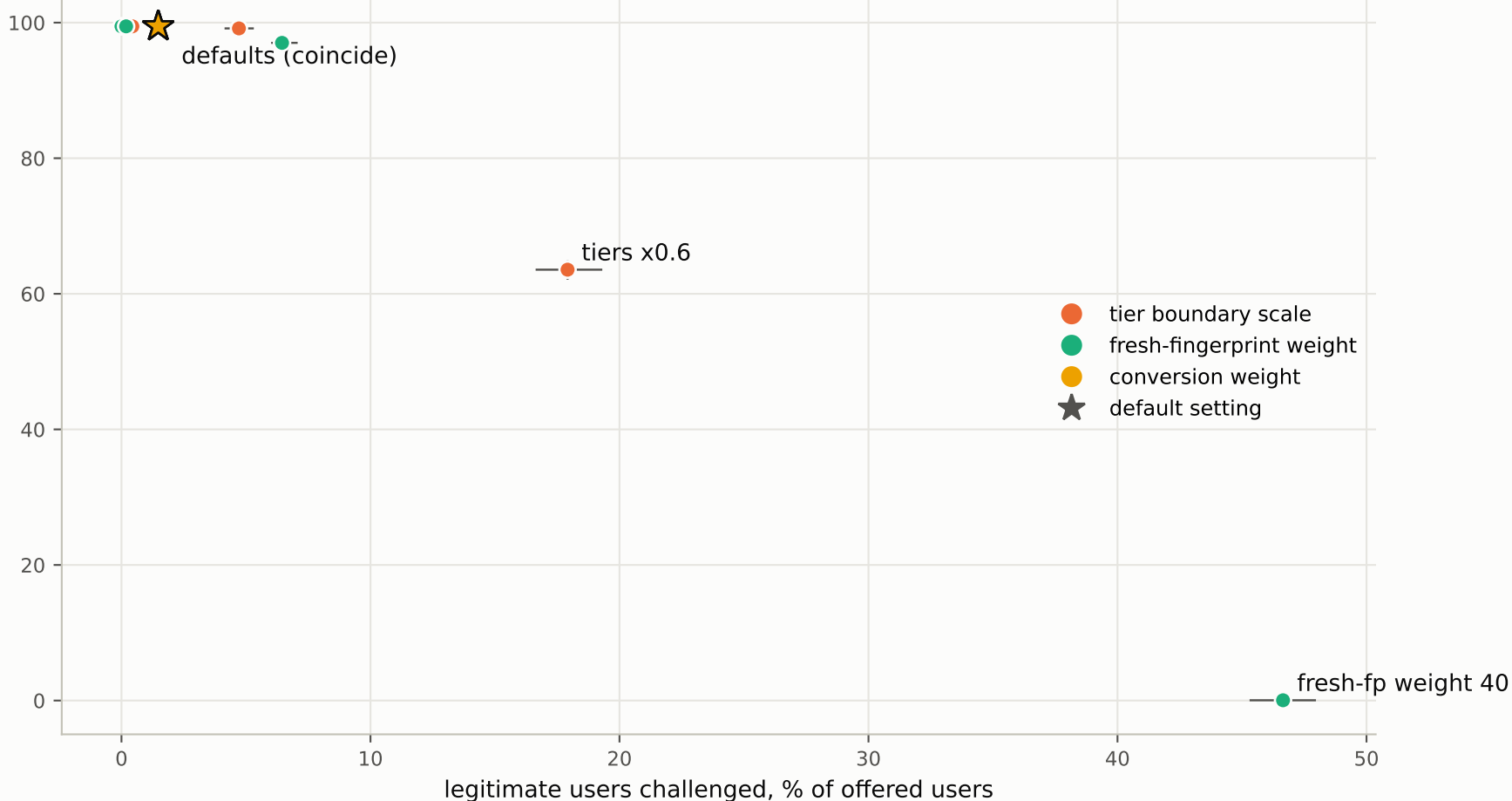
(b) risk-score settings, one at a time
