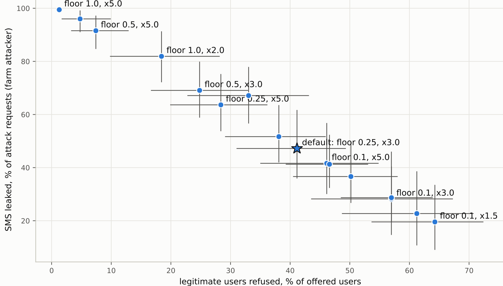
(b) risk-score settings, one at a time
